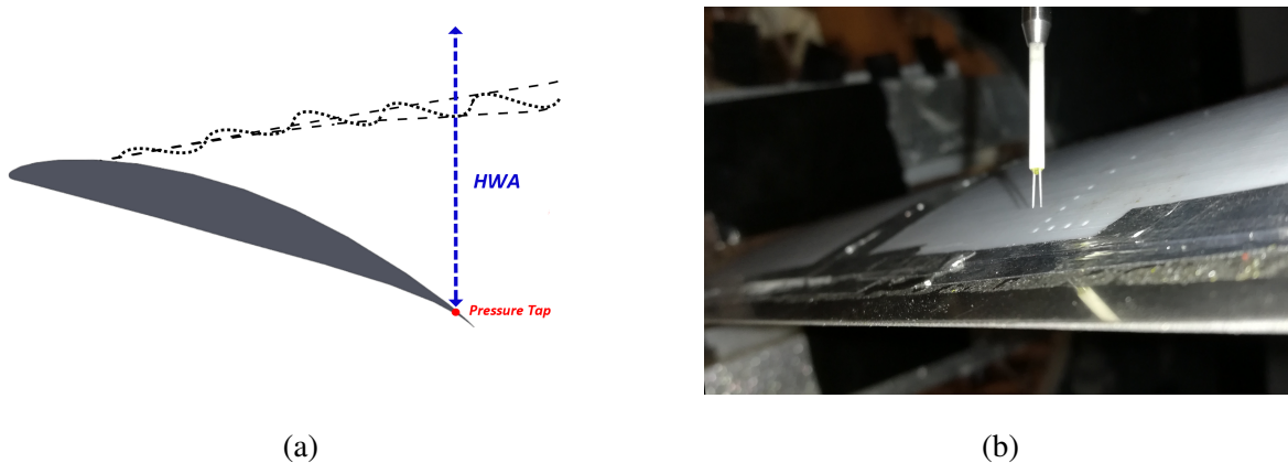
FIG. 13: Sketch and photo of the implementation of the simultaneous measurement of velocity (by means of Hot Wire Anemometry (HWA)) and surface pressure
