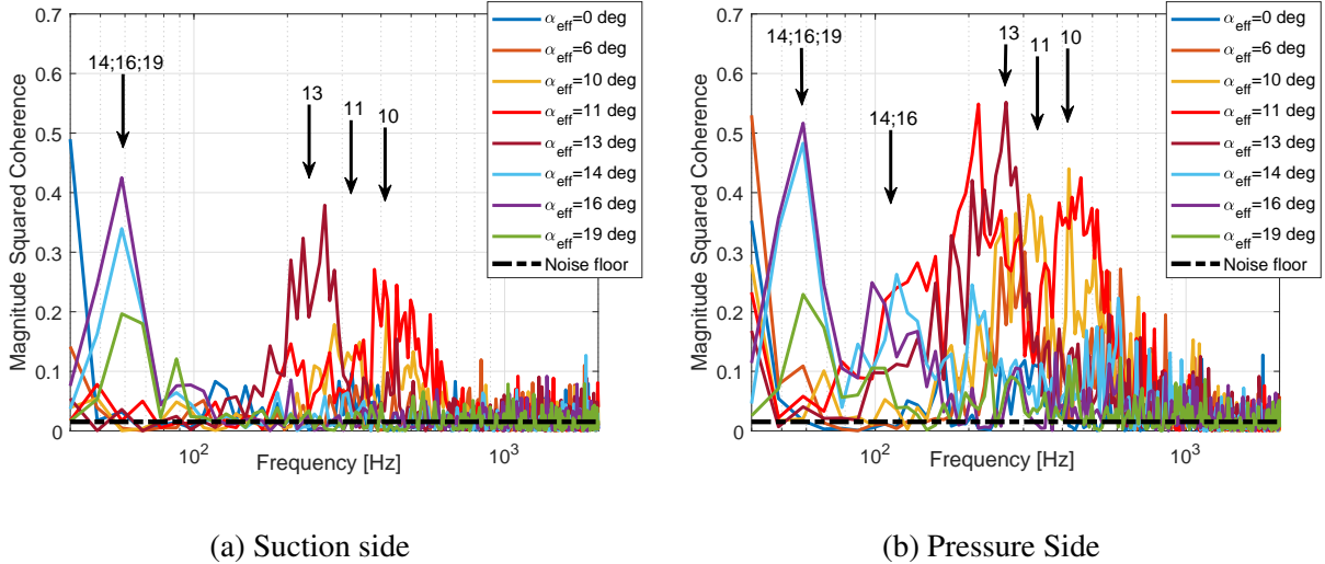
FIG. 9: Coherence between far field noise and surface pressure at TE for the NACA65(12)10 aerofoil at different angles of attack and U_\infty = 40m/s on a) Suction Side b) Pressure side; The dashed lines in a) and b) represent the statistical noise floor; The windowing was 4096 data-points.
