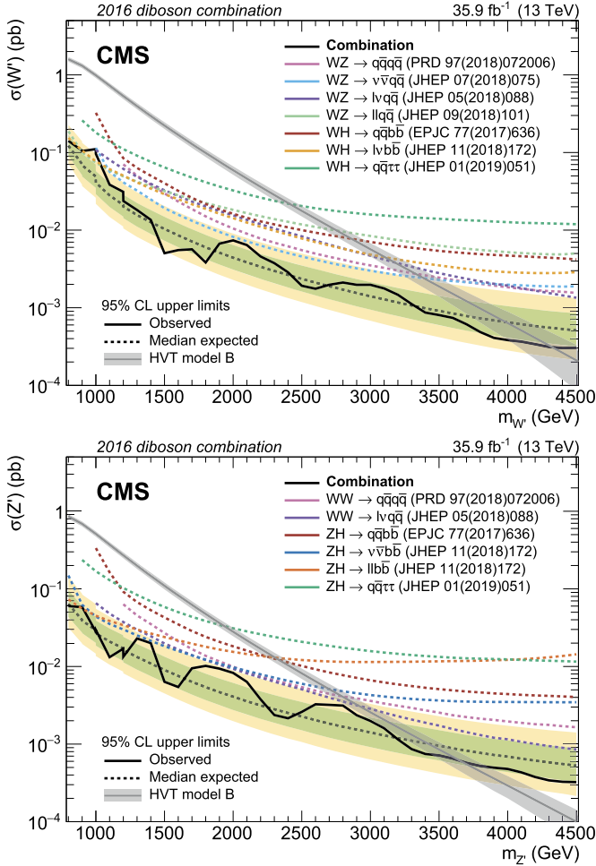
Fig. 2. Observed and expected 95% CL upper limits on the W' (upper) and Z' cross section (lower) as a function of the W' and Z' resonance mass. The inner green and outer yellow bands represent the \pm 1 and \pm 2 standard deviation variations on the expected limits of the statistical combination of the VV and VH channels considered. The expected limits in individual channels are represented by the colored dashed lines. The solid curves surrounded by the shaded areas show the cross sections predicted by the HVT model B and their uncertainties.
