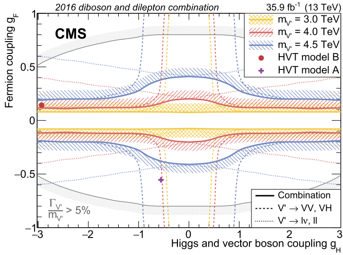
Fig. 4. Observed exclusion limits on the couplings of heavy vector resonances to fermions and SM vector bosons and the Higgs boson for the statistical combination of the dilepton (dotted lines) and diboson channels (dashed lines). Three resonance masses hypotheses (3.0, 4.0, and 4.5 TeV) are considered. The hatched bands indicate the regions excluded. The areas bounded by the thin gray contour lines correspond to regions where the resonance widths ( \Gamma_V ) are predicted to be larger than the average experimental resolution (5%).
