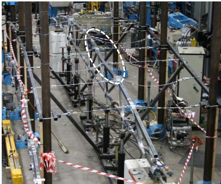
(b) Out-of-plane buckling of top chord of Truss 3
