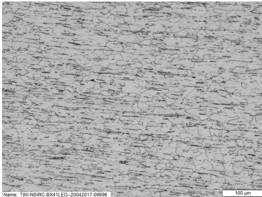
Figure 19: Micrograph of Mild Steel (S235) etched with 2% Nital
