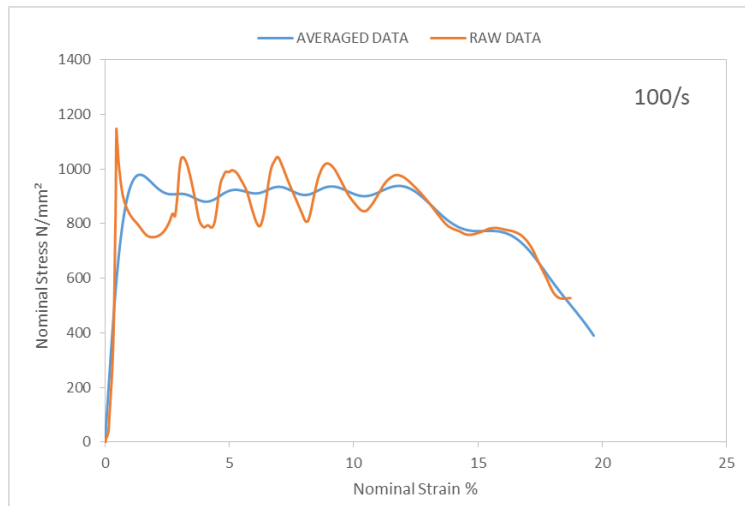
Figure 9: S960 result at strain rate of 100\text{s}^{-1}
