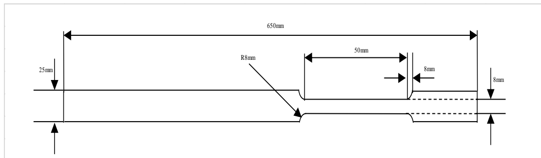
Figure 2: Quasi-static tensile test specimen geometry
