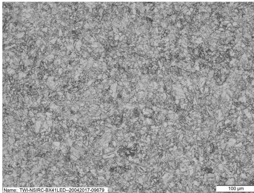
Figure 20: Micrograph of S690 etched with 2% Nital
