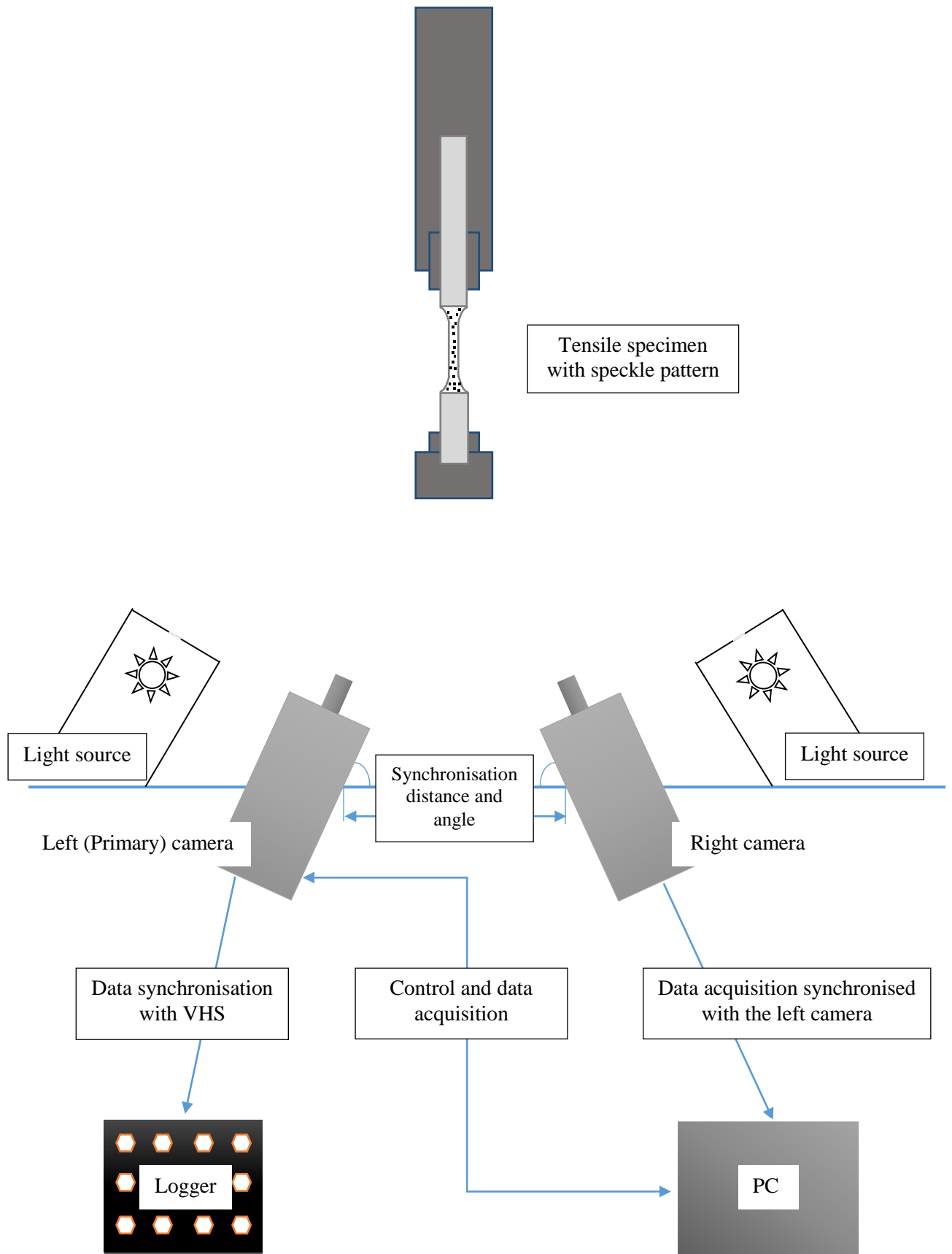
Figure 5: A simple schematic representation of the DIC setup and framework with the VHS machine.
