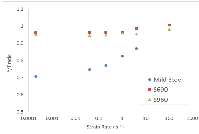
Figure 13: The effect of strain rate on the yield-to-tensile ratio of mild steel and high strength
