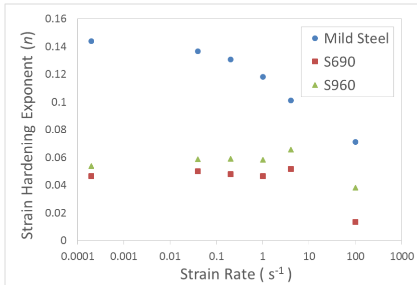
Figure 14: Effect of strain rate on the strain hardening exponent ( n ) of LSS (mild steel) and HSS
