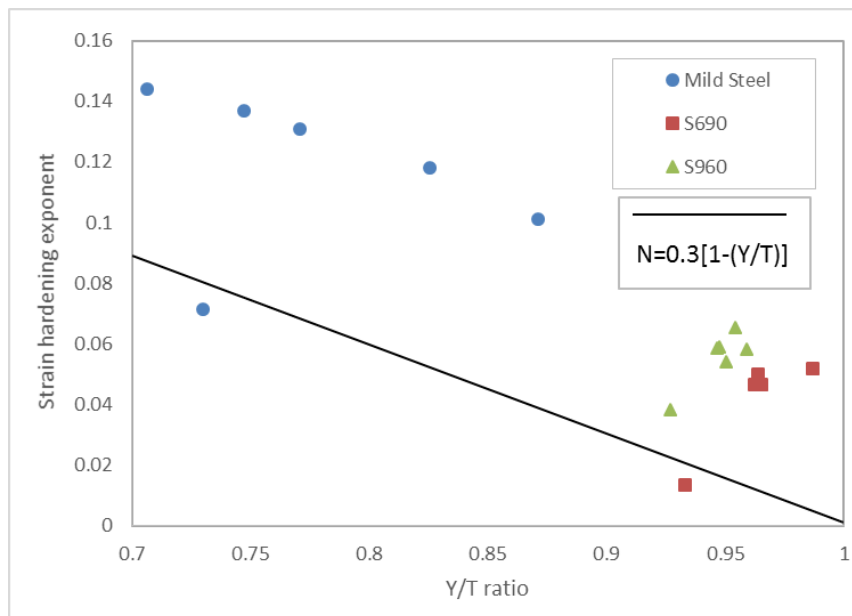
Figure 15: A conservative lower bound fit for calculating strain hardening exponent ( N ) from Y/T ratio using SINTAP approach, Eq. (5) [15]
