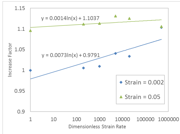
Figure 12: Flow stress increase factor ( \sigma_d/\sigma_0 ) dependence on the dimensionless strain rate ( \dot{\epsilon}_p/\dot{\epsilon}_0 ) for S960. Reference strain \dot{\epsilon}_0 taken as 2 \times 10^{-4} \text{ s}^{-1}
