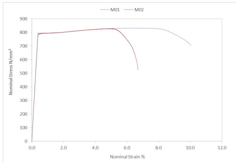
Figure 6: Effect of specimen geometry on S690 at quasi-static loading condition
