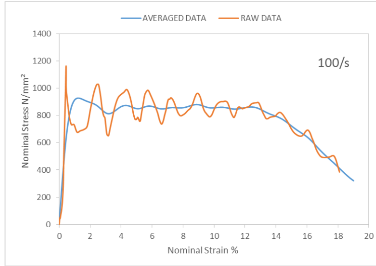
Figure 8: S690 result at strain rate of 100\text{s}^{-1}
