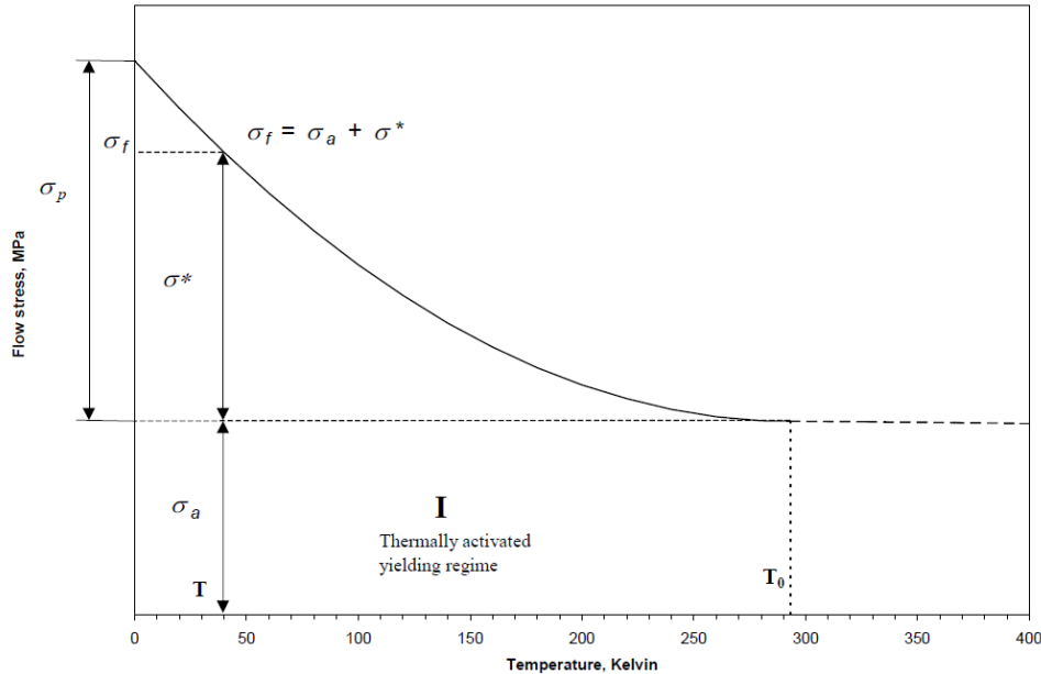
Figure 1: Flow stress partitions of an effective stress and internal stress with temperature of interest less 300 K [10]
