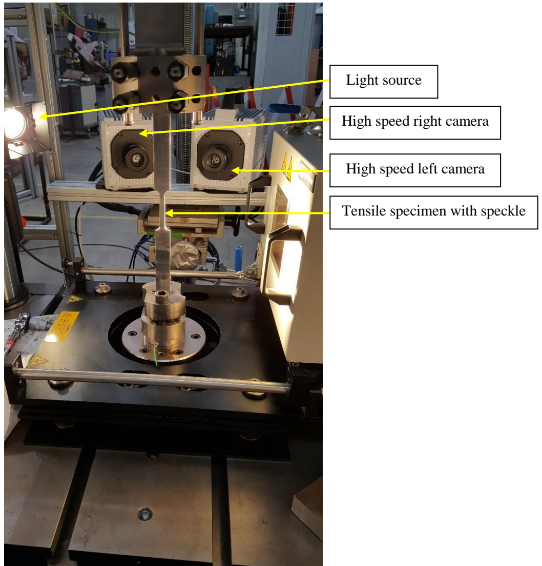
Figure 4: DIC system setup with the VHS test machine with view from behind (facing the camera)
