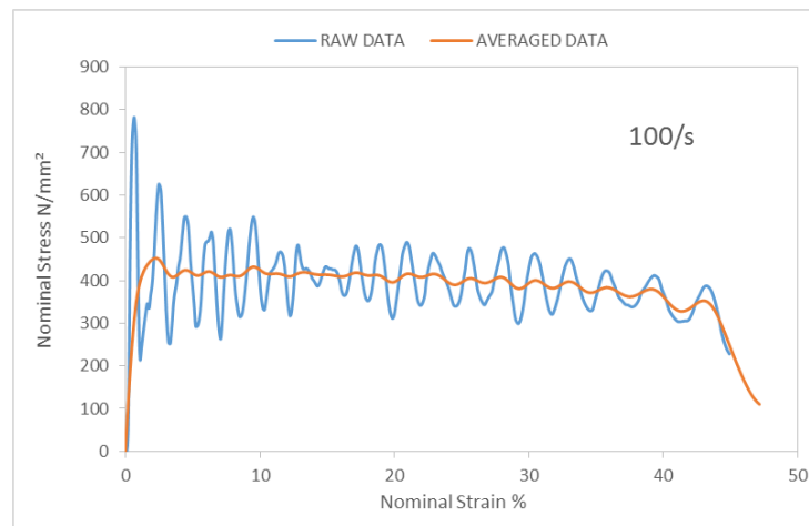
Figure 7: S235 result at strain rate of 100s -1
