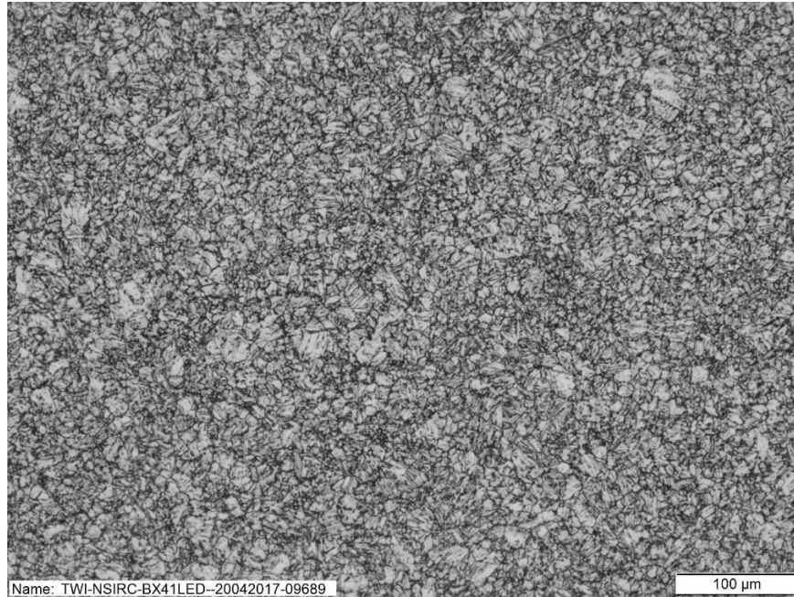
Figure 21: Micrograph of S960 etched with 2% Nital
