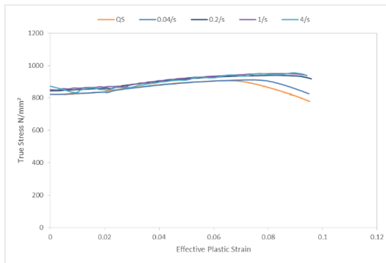
Figure 17: Flow stress for S690QL generated up to 4s^{-1} compared to QS results.
