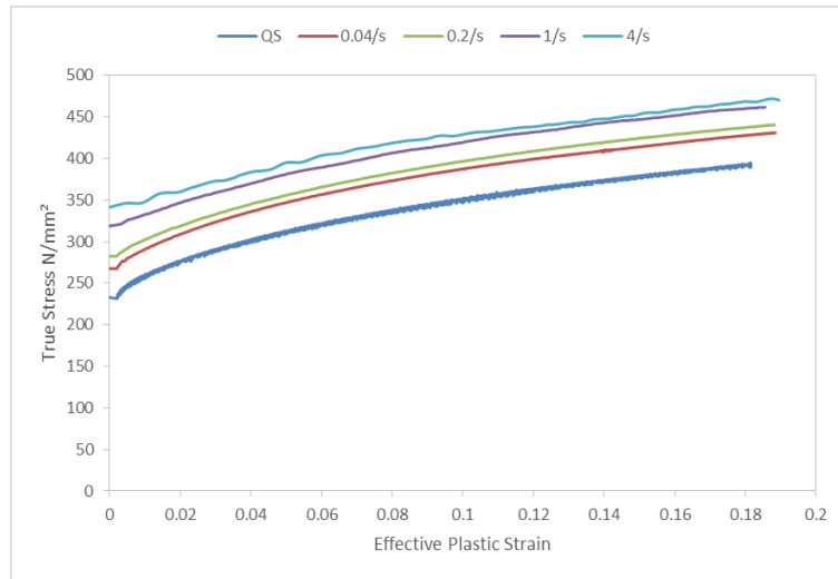
Figure 16: True stress-effective plastic strain for mild steel S235 up to 4s^{-1}
