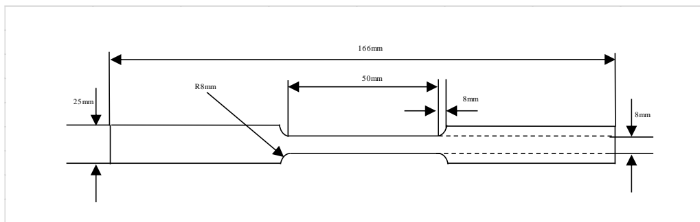
Figure 2: Quasi-static tensile test specimen geometry
