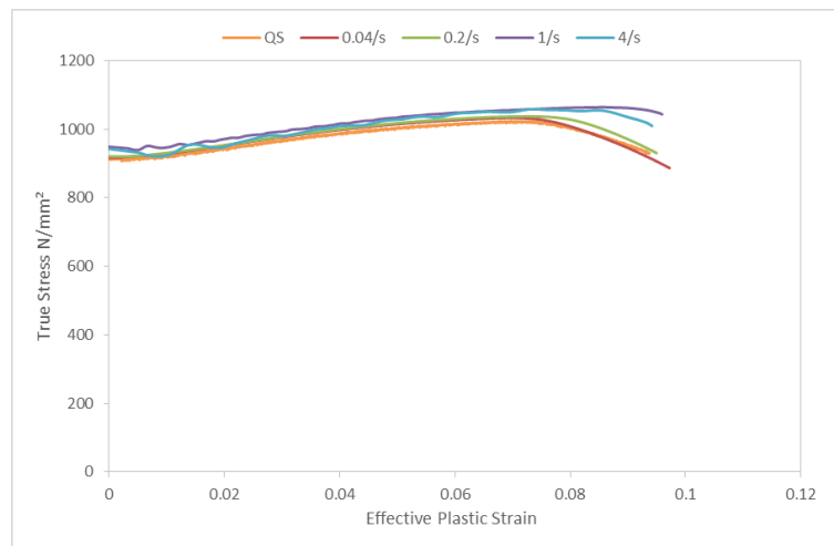
Figure 18: S960QL high strength steels generated up to 4s^{-1} QS results.
