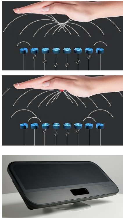
Figure 2: Top: Schematic illustration of principle of superposition to create a high-pressure haptic focus point. Bottom: STRATOS Inspire offers latest-generation mid-air haptics coupled with hardware suitable for public installations.
