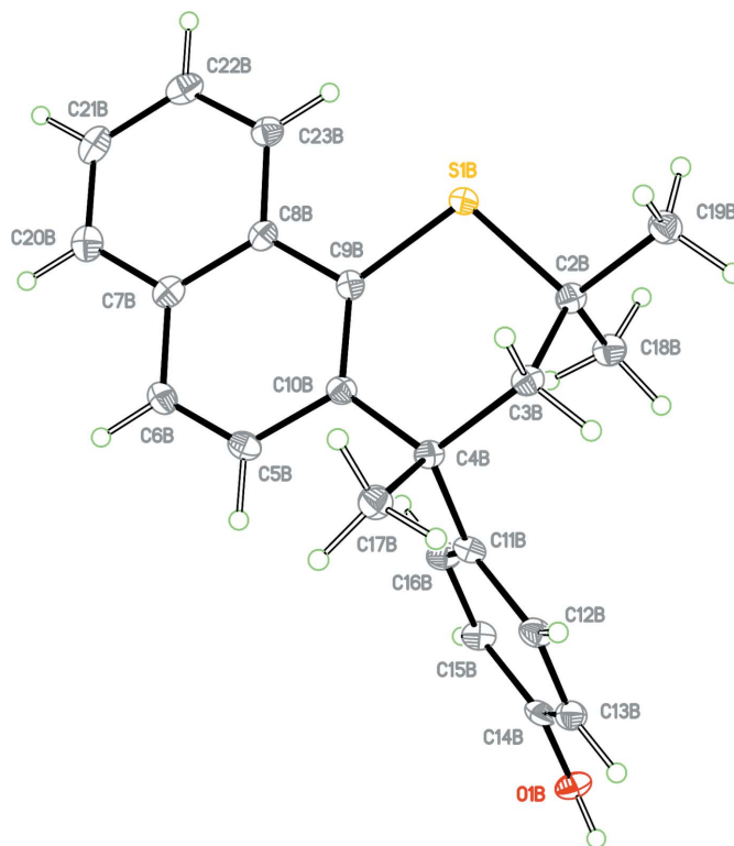
Figure 2 View of molecule B of the asymmetric unit with the atom labelling. Displacement ellipsoids are drawn at the 50% probability level.
