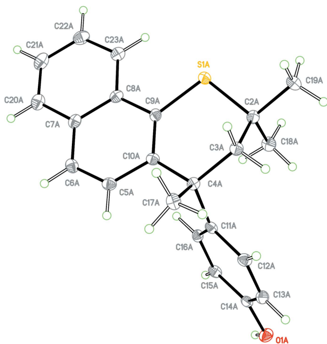
Figure 1 View of molecule A of the asymmetric unit with the atom labelling. Displacement ellipsoids are drawn at the 50% probability level.
