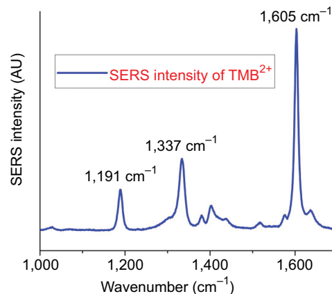
Figure S2 SERS spectra with characteristic Raman bands of TMB 2+ . Abbreviations: SERS, surface-enhanced Raman spectroscopy; TMB, 3,3',5,5'-tetramethylbenzidine.
