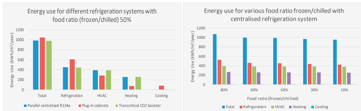
Fig. 2. (a) Energy use comparing three refrigeration systems for ratio frozen/chilled 50% (50% of all displayed products), (b) Total energy use and subsystems for various ratio of frozen/chilled with the centralised refrigeration system
