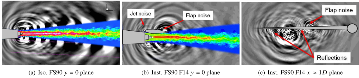
Fig. 26 Instantaneous dp/dt contours for the isolated and F14 case at different plane locations with axial velocity contours in the jet plume region.
