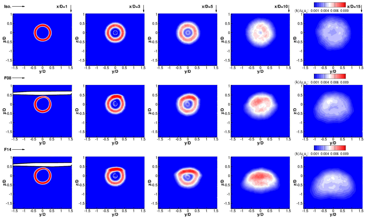
Fig. 12 Turbulence kinetic energy contours \langle k \rangle / u_c^2 at different x -planes. Rows represent cases, columns represent axial plane locations as labelled.
