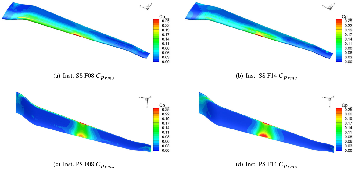
Fig. 22 Flap suction and pressure side C_{p_{rms}} contours.
