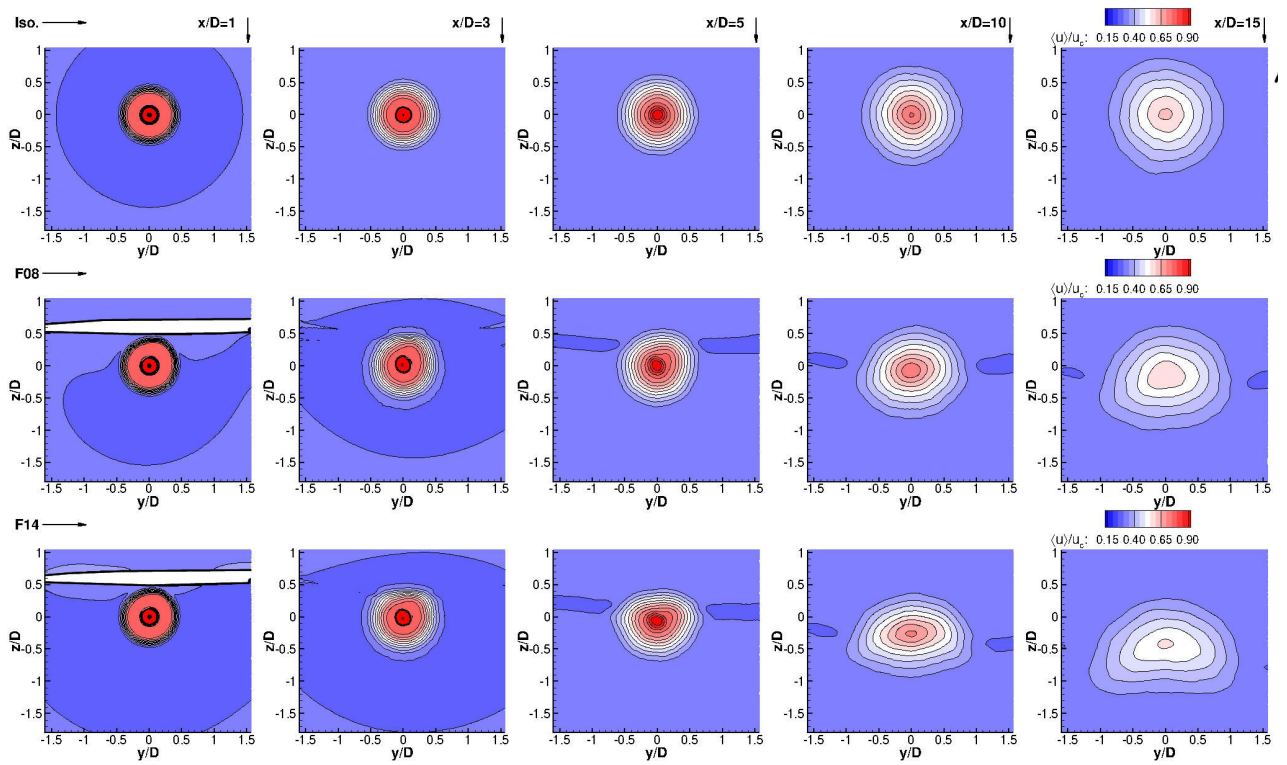
Fig. 9 Axial velocity contours \langle u \rangle / u_c at different x -planes. Rows represent cases, columns represent axial plane locations as labelled.
