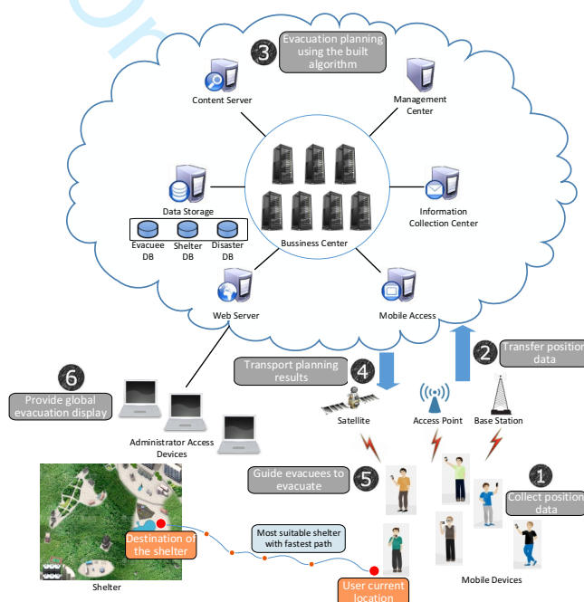
Fig. 1. The system architecture of CLOTHO
