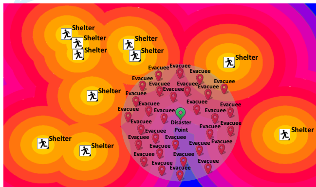
Fig. 5. The model of the emergency evacuation planning scenario based on the artificial potential field.
