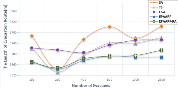
Fig. 11. The average length of evacuation route. (a) Under the condition of capacity remaining. (b) Under the condition of insufficient capacity.
