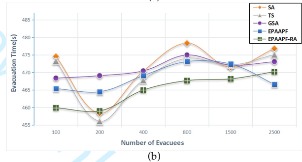
Fig. 12. The average evacuation time. (a) Under the condition of capacity remaining. (b) Under the condition of insufficient capacity.
