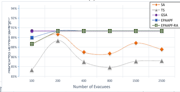
Fig. 13. The algorithm running accuracy of different capacity. (a) Under the condition of capacity remaining. (b) Under the condition of insufficient capacity.
