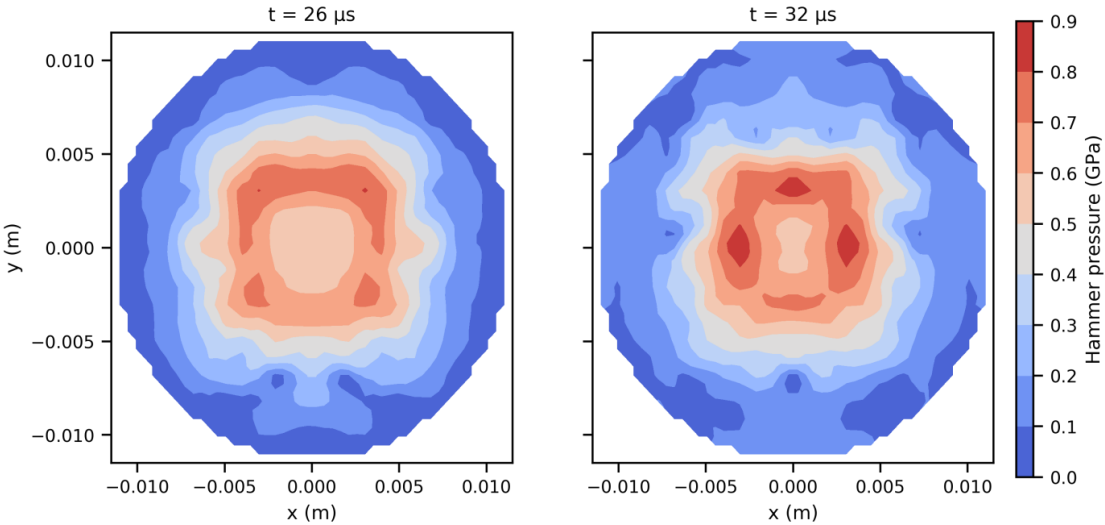
Figure 6: Hammer pressure contour on the surface of specimen at t = 26 \mu s and t = 32 \mu s
