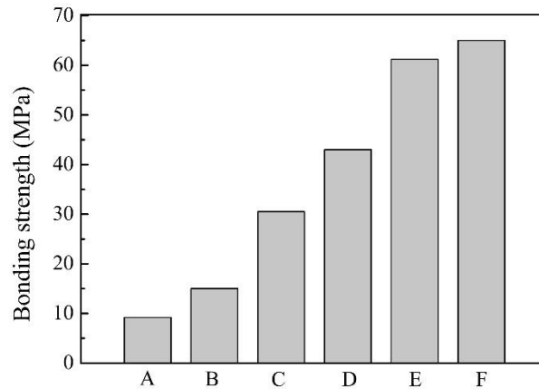
Figure 10: Bonding strength of different thermal sprayed coatings: A [52]: plasma sprayed hydroxyapatite, B [53]: plasma sprayed YSZ, C [54]: plasma sprayed Ni 20 Cr, D [55]: HVOF sprayed Fe-based amorphous composite, E [54]: plasma sprayed Ni 20 CrMo and F [56] plasma sprayed Al-Si and B 4 C composite
