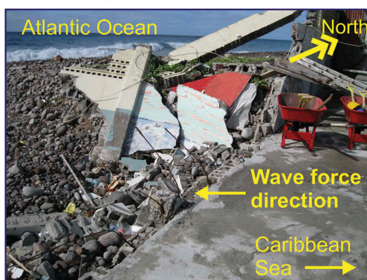
Figure 7. Different types of damage to coastal structures from Hurricane Maria in Dominica, observed during the field survey (part 1).
