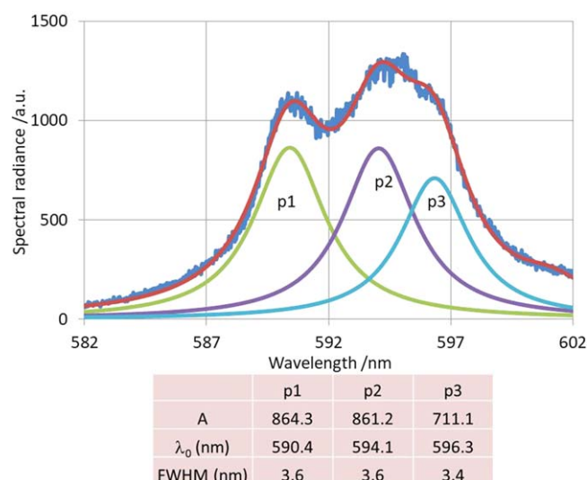
Figure 6. Deconvolution of ^{5}D_0 \rightarrow ^{7}F_1 transitions of \text{Eu}^{3+} in S20 NDs recorded at 0 °C. Deconvolution was achieved with three Lorentzian profiles, which were fitted to the experimental spectrum with a least squares algorithm using the solver of Excel Microsoft.
