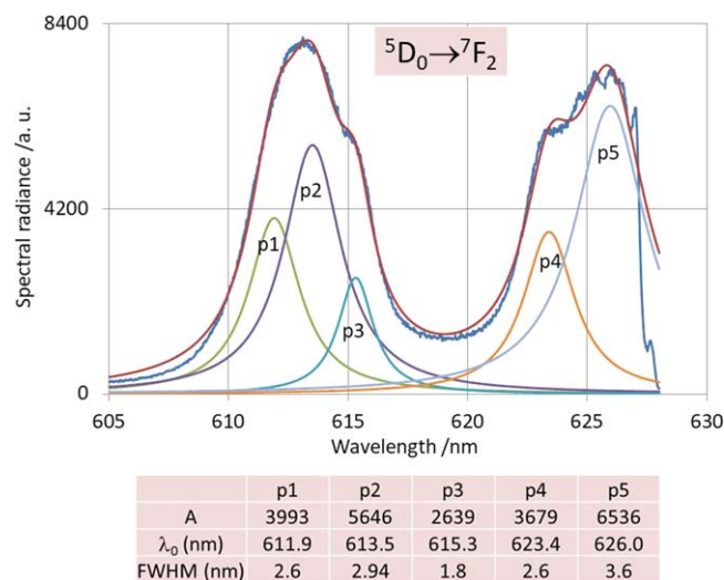
Figure 7. Deconvolution of ^{5}D_0 \rightarrow ^{7}F_2 transitions of \text{Eu}^{3+} in S20 NDs recorded at 0 °C. Deconvolution was achieved with five Lorentzian profiles, which were fitted to the experimental spectrum with a least squares algorithm using the solver of Microsoft Excel.
