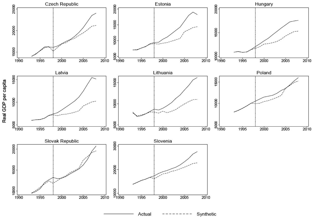
Fig. 5. Actual vs. synthetic country – GDP per capita trends, eastern enlargement (1998 anticipation). Note: In each graph, the continuous line represents the trend of the real GDP per capita (PPP, 2005 International Dollars) for the actual country, while the dashed line shows the trend for the same variable for the synthetic country. For each country the analysis ends in 2008. The composition of each synthetic country is reported in Figure 4 and full details in Table A.3 in Appendix.
