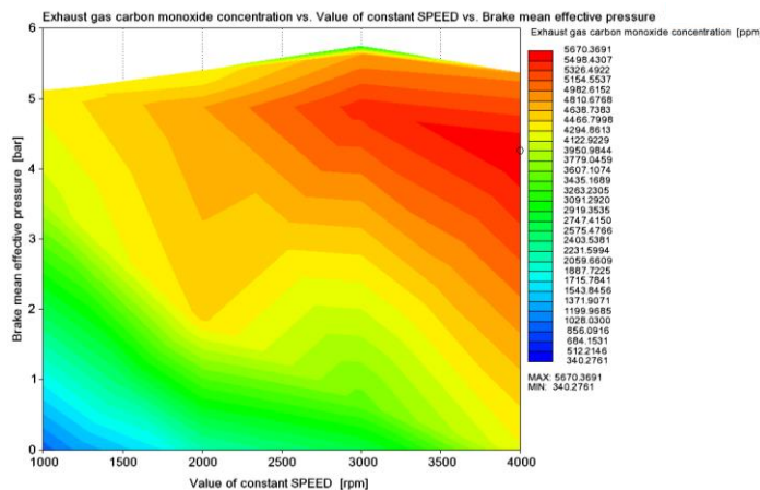
Figure 13 Part load CDA+VVA CO emission (ppm)
