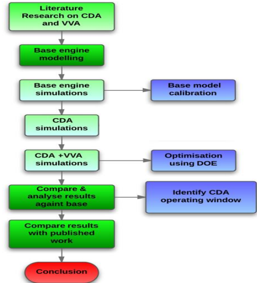
Figure 2 Methodology flowchart
