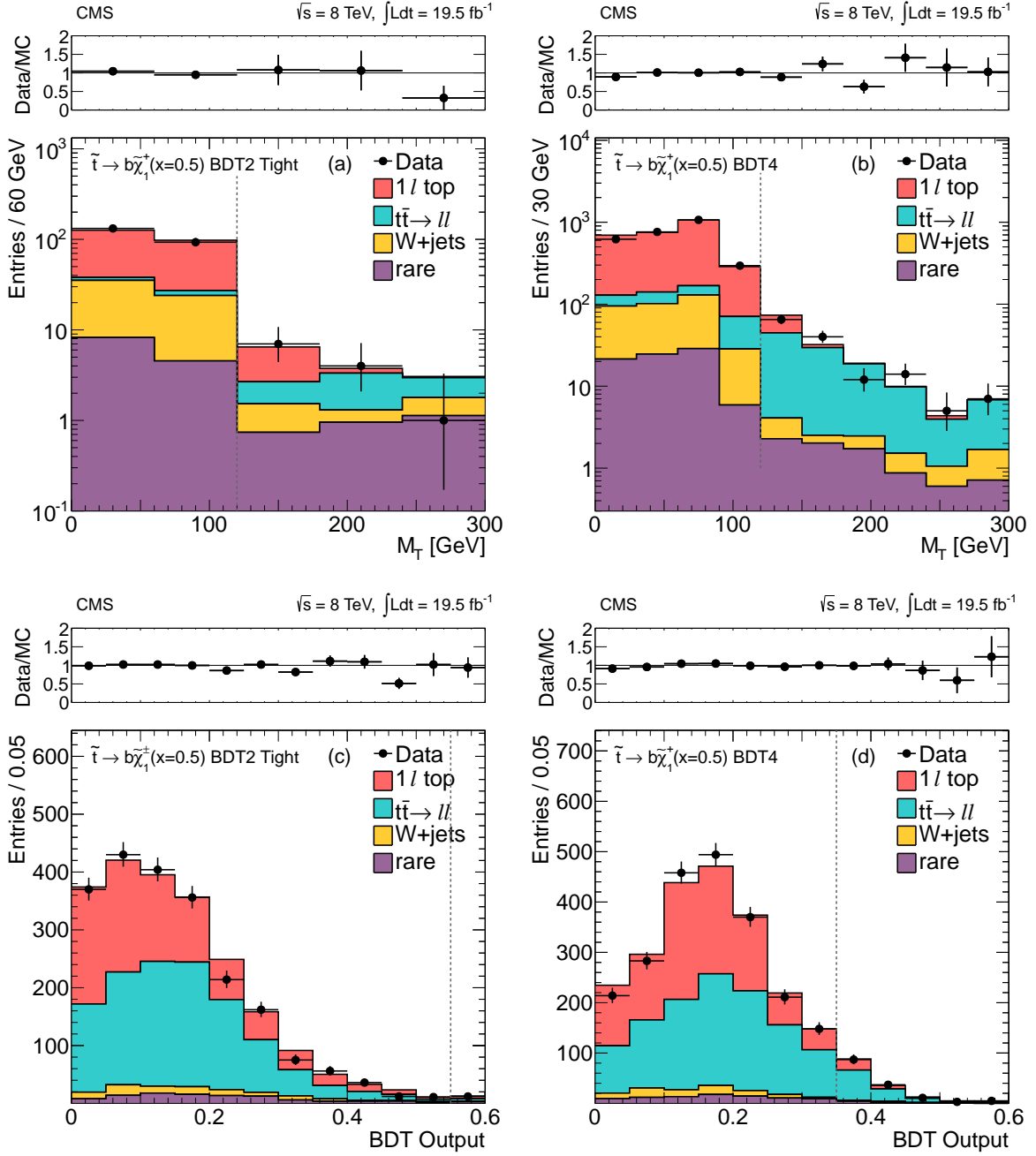
Figure 17: Comparison of data and MC simulation for the distributions of BDT output and M_T corresponding to the x = 0.5 \tilde{t} \rightarrow b \tilde{\chi}_1^+ scenario in training regions 2 and 4. The M_T distributions are shown after the requirement on the BDT output, and the BDT output distributions are shown after the M_T > 120 GeV requirement (these requirements are also indicated by vertical dashed lines on the respective distributions). (a) M_T after the tight cut on the BDT2 output; (b) M_T after the cut on the BDT4 output; (c) BDT2 output after the M_T cut; (d) BDT4 output after the M_T cut. In all distributions the last bin contains the overflow.
