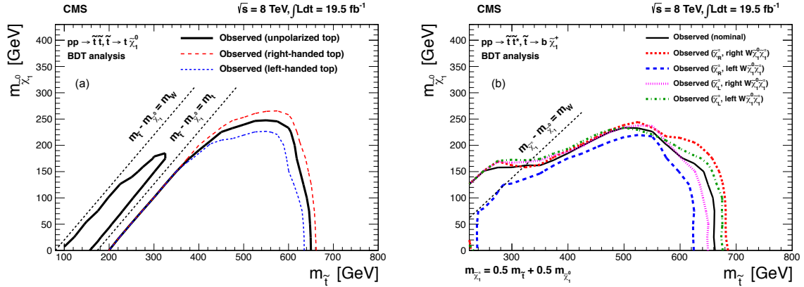
Figure 11: (a) the observed 95% CL excluded regions for the \tilde{t} \rightarrow t\tilde{\chi}_1^0 model for the case of unpolarized, right-handed, and left-handed top quarks. (b) the observed 95% CL excluded regions for the \tilde{t} \rightarrow b\tilde{\chi}_1^+ model with x = 0.5 for the nominal scenario, right- vs. left-handed charginos ( \tilde{\chi}_R^\pm and \tilde{\chi}_L^\pm , respectively), and right- vs. left-handed W\tilde{\chi}_1^\pm \tilde{\chi}_1^\pm couplings.
