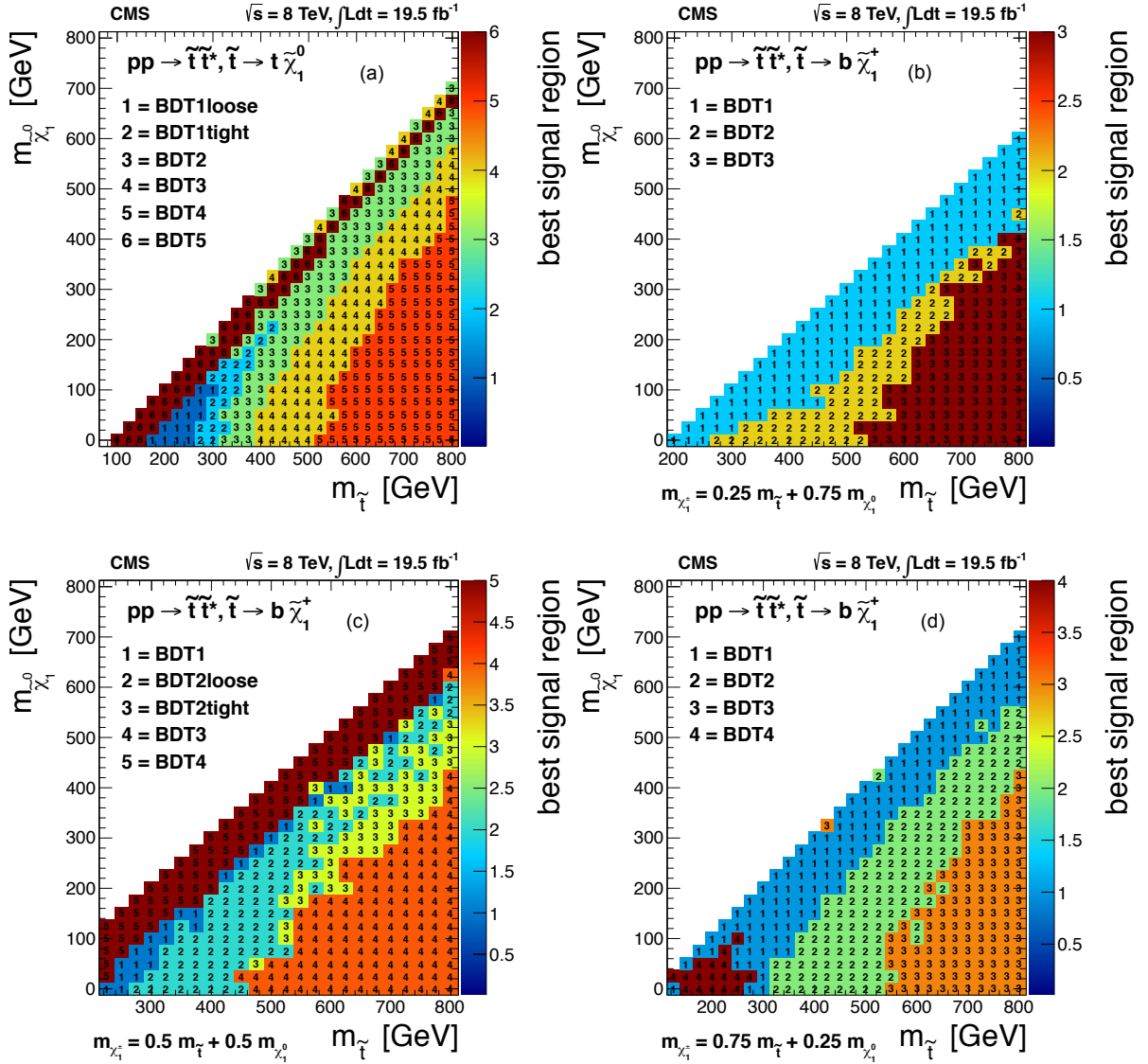
Figure 21: The most sensitive signal region in the m_{\tilde{\chi}_1^0} vs. m_{\tilde{t}} parameter space in the BDT analysis, for the (a) \tilde{t} \rightarrow t\tilde{\chi}_1^0 model, and the \tilde{t} \rightarrow b\tilde{\chi}_1^+ model with chargino mass parameter (b) x = 0.25 , (c) 0.5, and (d) 0.75. The number indicates the BDT training region.
