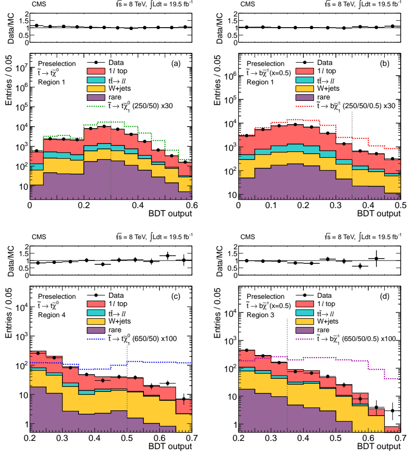
Figure 4: Comparison of data and MC simulation for sample BDT outputs. (a) \tilde{t} \rightarrow t\tilde{\chi}_1^0 scenario in training region 1; (b) \tilde{t} \rightarrow b\tilde{\chi}_1^{\pm} scenario with x = 0.5 in training region 1; (c) \tilde{t} \rightarrow t\tilde{\chi}_1^0 scenario in training region 4; (d) \tilde{t} \rightarrow b\tilde{\chi}_1^{\pm} scenario with x = 0.5 in training region 3. Only the event preselection is applied, and in all cases the last bin contains the overflow. Events in the signal regions are further selected by requiring M_T > 120 GeV and by applying BDT requirements as indicated by the vertical dashed lines. We also overlay expectations for possible signals with m_{\tilde{t}} = 250 GeV and m_{\tilde{\chi}_1^0} = 50 GeV (panels (a) and (b)) and m_{\tilde{t}} = 650 GeV and m_{\tilde{\chi}_1^0} = 50 GeV (panels (c) and (d)). For display purposes, these are scaled up by factors of 30 and 100 respectively.
