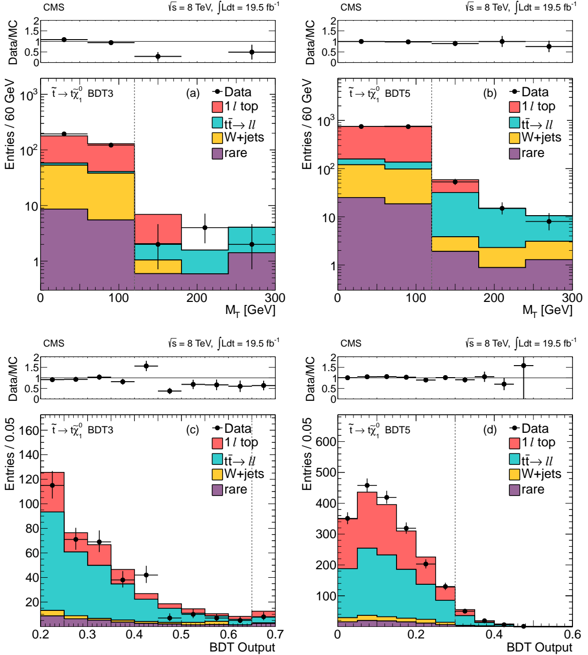
Figure 14: Comparison of data and MC simulation for the distributions of BDT output and M_T corresponding to the \tilde{t} \rightarrow t\tilde{\chi}_1^0 scenario in training regions 3 and 5. The M_T distributions are shown after the requirement on the BDT output, and the BDT output distributions are shown after the M_T > 120 GeV requirement (these requirements are also indicated by vertical dashed lines on the respective distributions). (a) M_T after the cut on the BDT3 output; (b) M_T after the cut on the BDT5 output; (c) BDT3 output after the M_T cut; (d) BDT5 output after the M_T cut. In all distributions the last bin contains the overflow.
