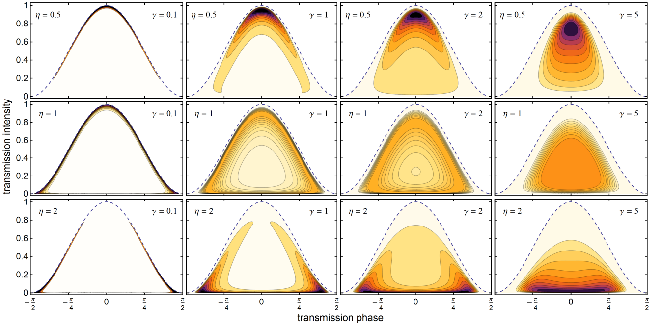
FIG. 1. Contour plots of the joint distribution (12) of the transmission intensity ( T ) and phase ( \theta ) at the background coupling \eta = 0.5, 1, 2 (rows) and absorption rates \gamma = 0.1, 1, 2, 5 (columns). Darker regions correspond to higher values of the jpdf, with black standing for the values of 40, 5, 3.5, 3 at \gamma = 0.1, 1, 2, 5 , respectively. The dashed line indicates the boundary T = \cos^2 \theta of the distribution support.
