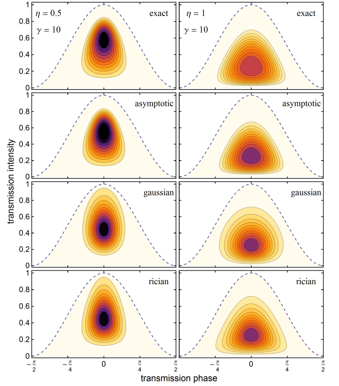
FIG. 2. Comparison between the exact jpdf (12), its asymptotic form (14) and the Gaussian (15) and Rician (18) approximations at strong absorption. The background coupling \eta = 0.5 (left panel) or 1 (right panel) and the absorption rate \gamma = 10 everywhere.
