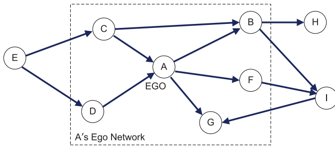
Fig. 9: Ego Network
