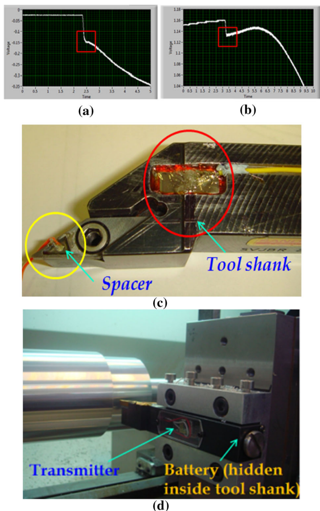
Figure 4 a Voltage output from smart tool 1; b voltage output from smart tool 2; c smart tool 2; d cutting trails illustration
