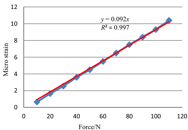
Figure 11 Correlation between static force and strain output
