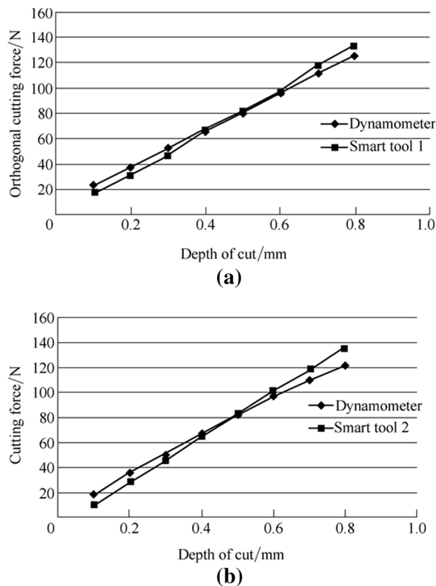
Figure 5 Cutting force measurement with a smart tool 1, b smart tool 2, and calibration against Kistler dynamometer
