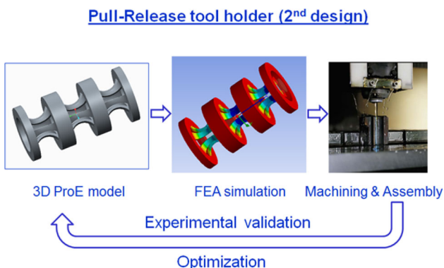
Figure 17 Design of the pull-release tool collet for high speed micro drilling spindles
