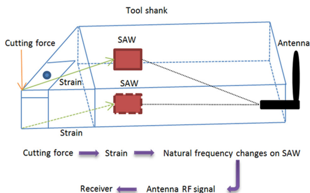
Figure 6 Schematic illustration of the principle using SAW sensors on the tool shank to detect cutting forces
