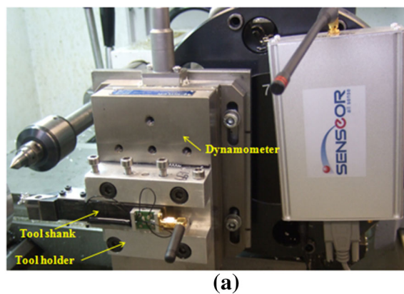
Figure 10 SAW strain sensors instrumented onto the cutting tool shank
