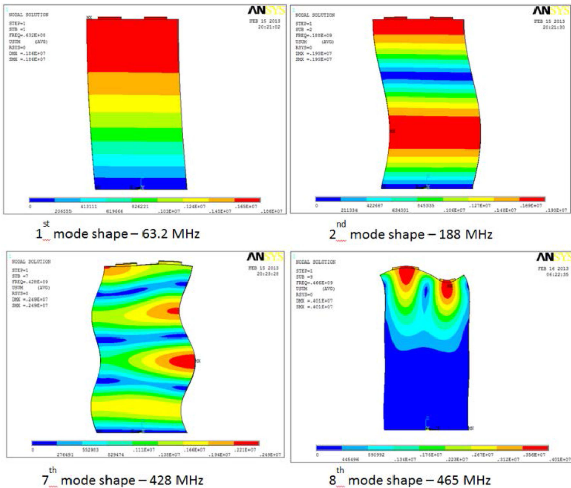
Figure 8 The 8th mode shape at 465 MHz and other modes for the SAW sensors
