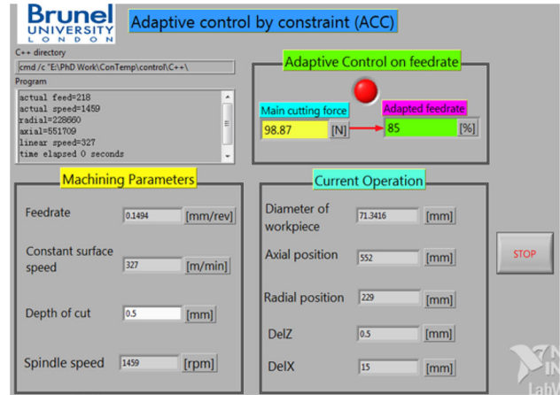
(a) System interface programmed in LabVIEW
