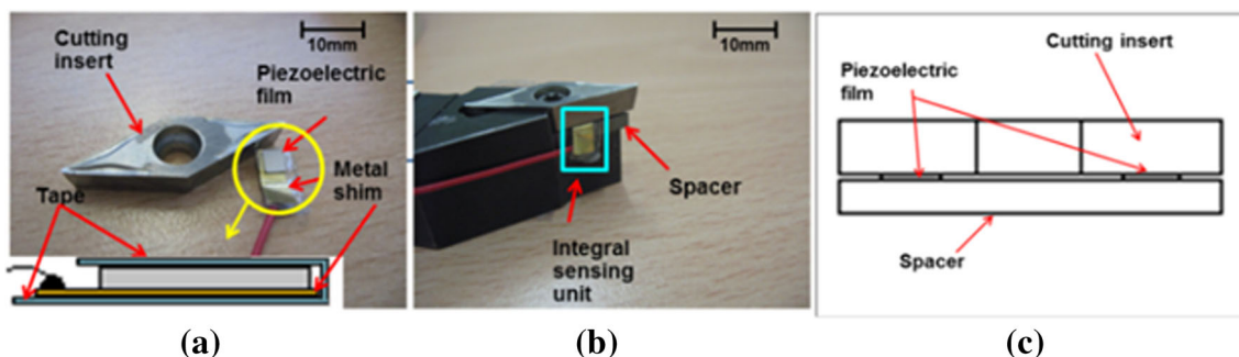
Figure 2 a Composition of the smart cutting tool; b assembly of the tool; c cross section view of the tool
