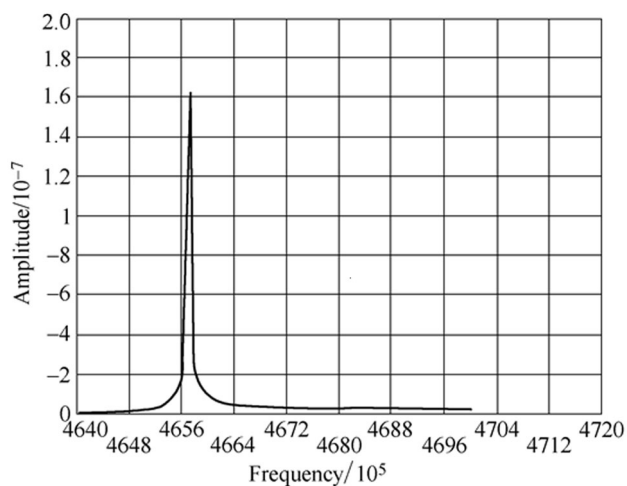
Figure 9 Frequency response of the SAW in the harmonic analysis
