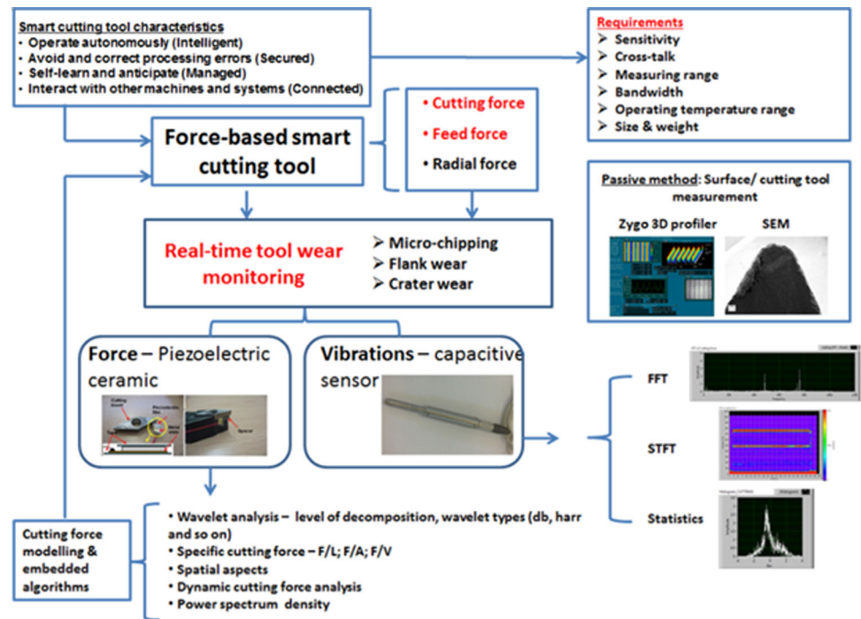
Figure 3 Illustration of the smart tool development protocol
