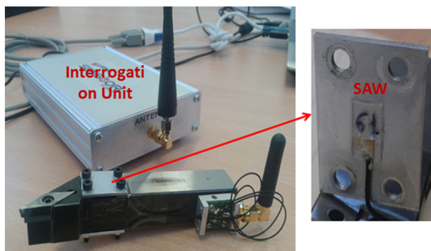
Figure 10 SAW strain sensors instrumented onto the cutting tool shank
