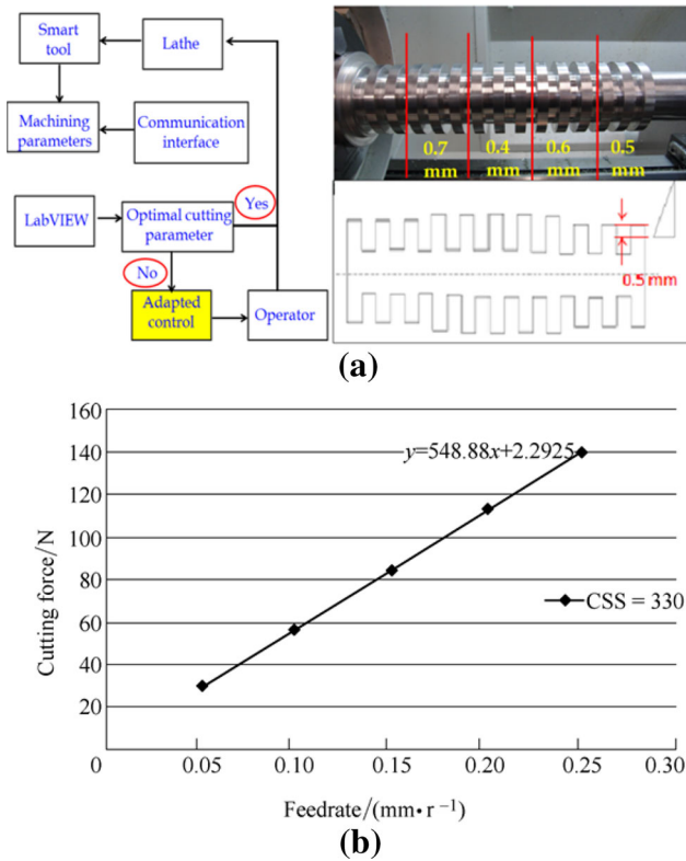
Figure 18 a Adaptive control loop and adaptive smart machining trails on a CNC machine; b the relationship between the federate and cutting force
