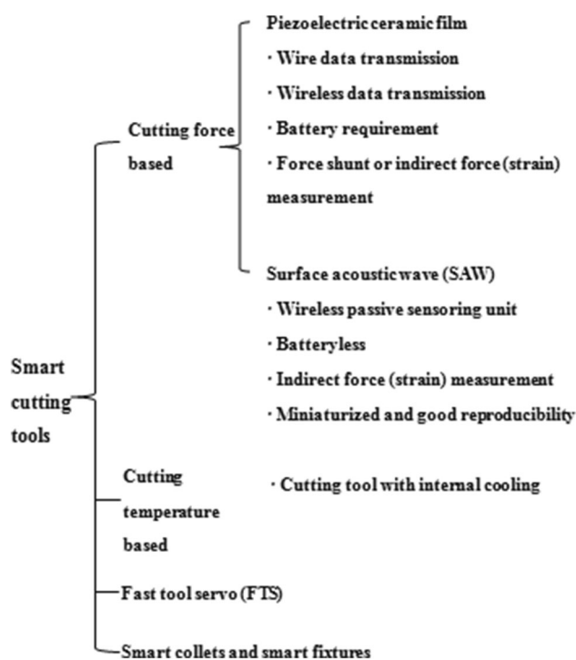
Figure 1 Family schematic of smart cutting tools
