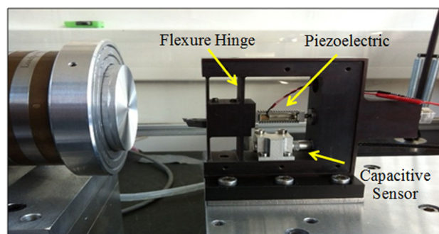
Figure 14 Fast tool servo mounted on the micro turning machine
