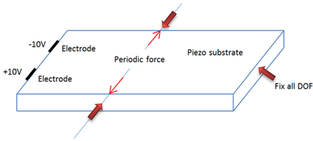
Figure 7 Boundary conditions defining the propagation for the FEA simulations
