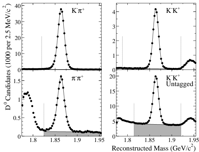
FIG. 1: The reconstructed D^0 mass distribution (points) superimposed on a projection of the mass fit (curve) for the four D^0 samples. The fit was performed within the restricted ranges of mass indicated by the vertical dotted lines. The portion of the sample assigned by the fit to the background is indicated by the shaded region.
