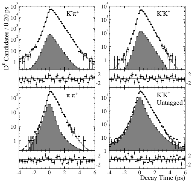
FIG. 2: The decay-time distribution for the four D^0 samples (points) within a \pm 15 MeV/ c^2 mass signal window superimposed on a projection of the lifetime fit (histogram). The shaded histogram is the portion of the sample assigned by the fit to the background. The points presented below the histograms are the difference between data and fit divided by the statistical error with error bars of unit length.
