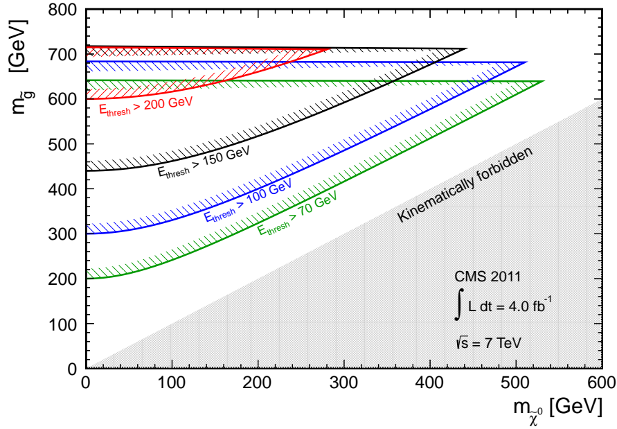
Figure 5: The region of m_{\tilde{g}} - m_{\tilde{\chi}_0^0} excluded by the analysis, valid for gluino lifetimes 10^{-5} \text{ s} < \tau_{\text{gluino}} < 10^3 \text{ s} , using several jet energy thresholds E_{\text{thresh}} .
