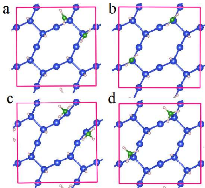
Figure 5. Schematic structures and formation energies of two BH 2 clusters: (a) on top of two bridging Si atoms (close to each other), (b) on two separated surface Si atoms, (c) on two BH 3 clusters on two bridging Si atoms, and (d) on two separated Si atoms. It is noted the calculations showed that all the configurations are stable with respect to the H-passivated surface and BH 3 molecules (Equations 2 and 3). The most stable one is two BH 3 clusters on two bridging Si atoms/ions. Structure optimizations showed that Si-Si bond between the bridging Si atoms/ions is broken due to the BH 3 deposition (Figure 5c).
