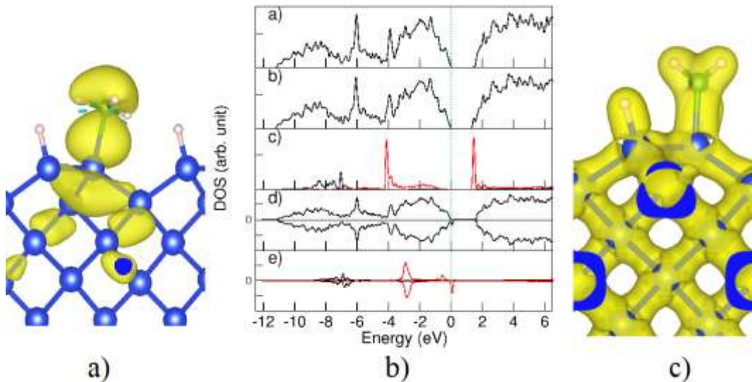
Figure 2. (a) Spin density iso-surface for one BH_3 on a Si(100) surface, (b) total and partial density of states (DOS) for the selected systems: (b_a) total DOS for the Si(001) 2\times 1:H surface; (b_b) total DOS for the surface with a BH_2 radical; (b_c) partial DOS for the B in the radical; (b_d) total DOS for the surface with a BH_3 radical; (b_e) partial DOS for the B in the radical, and (c) electron density iso-surface for one BH_2 radical on the Si(100) surface. In Figures 1b_c and 1b_e, the black curves represent the partial DOS for the B-2s characters, and the red curves represent the B-2p states.
