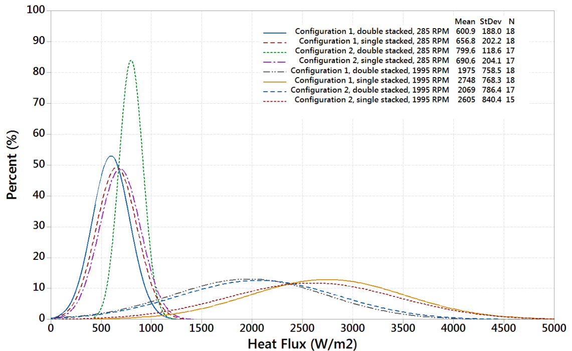
Distribution of Heat Flux (W/m 2 )
