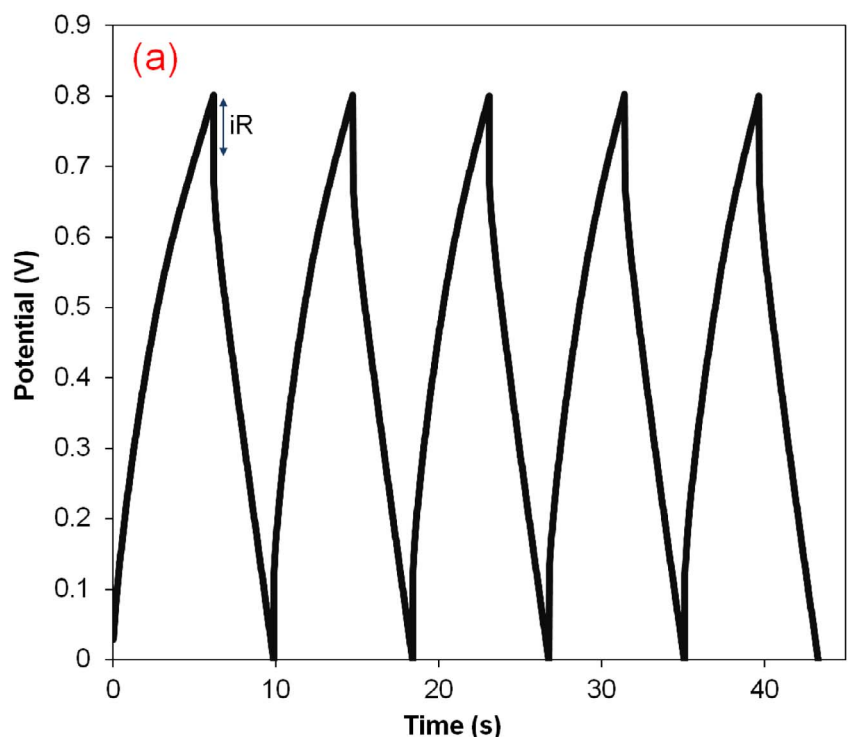
Fig. 6. (a) Constant current GCD curve of flexible electrodes at current of 15 mA; (b) GCD curve recorded at different charge currents.
