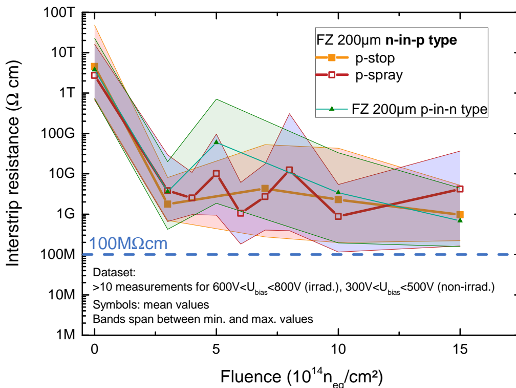
Figure 7. Interstrip resistance to the neighboring strip vs. irradiation fluence for nominal 200\mu\text{m} thick sensors. The resistance is normalized to 1\text{cm} strip length. Each data point indicates the mean of at least ten measurements (different strips on same sensor) on fully depleted sensors. The bands indicate the maximum and minimum values measured. Measurements on non-irradiated samples were performed at room temperature, else at -20^\circ\text{C} .
