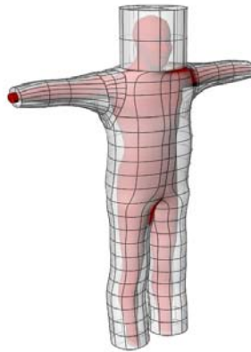
Fig. 4. Reconstruction geometry for worker/suit combination of fig. 3
