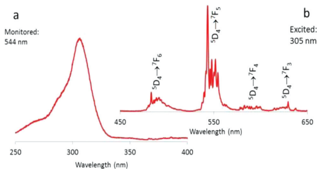
Fig. 16 Excitation (a) and emission spectra (b) of Lu_2O_3:0.1\%Tb^{3+} . Vertical scales are linear and represent intensity in arbitrary units. The {}^5D_3 \rightarrow {}^7F_J transitions at \lambda < 475\text{ nm} are too weak to be detected.
