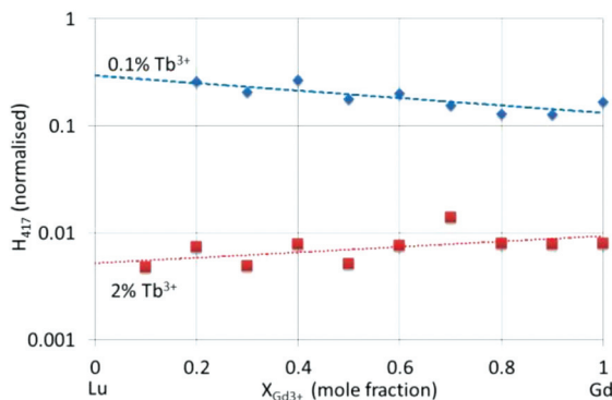
Fig. 14 Maximum normalised peak height of the {}^5D_3 \rightarrow {}^7F_5 transition ( H_{417} ) versus the composition parameter x of (Lu_{1-x}Gd_x)_2O_2S:Tb^{3+} . The excitation wavelength was 292 nm.
