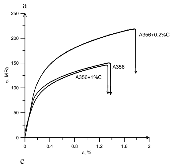
Figure 2. Introduction of nanodiamond particles to an A356 matrix: a, b, OM microstructures showing the distribution of nanoparticles in an A356–0.2 wt% C MMNC; c, tensile curves showing improved strength and ductility at 0.2 wt% addition.
