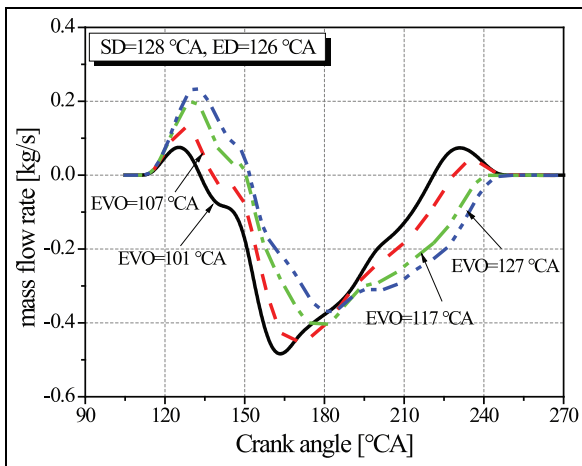
Figure 17. The total mass flow rate profiles at the outlets of scavenge ports for different EVOs (SD = 128 °CA, ED = 126 °CA).
