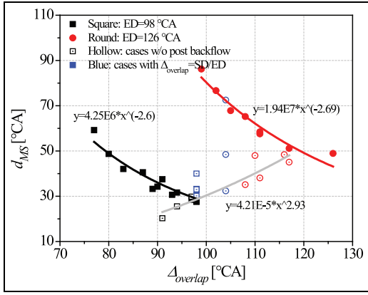
Figure 28. Correlation of d_{MS} with \Delta_{overlap} .
