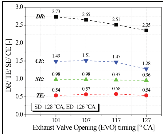
Figure 19. Effect of EVO on DR, TE, SE and CE (SD = 128 °CA, ED = 126 °CA).
