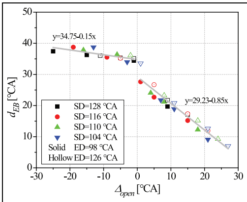
Figure 25. Correlation of d_{EB} with \Delta_{open} .
