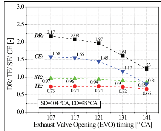
Figure 21. Effect of EVO timing on DR, TE, SE and CE (SD = 104 °CA, ED = 98 °CA).
