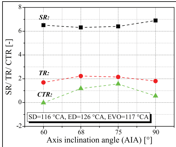
Figure 4. Effect of AIA on in-cylinder flow motions (SD = 116 °CA, ED = 126 °CA, EVO = 117 °CA).
