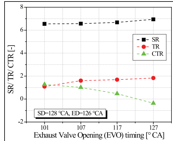
Figure 18. Effect of EVO on the SR, TR and CTR at 280 °CA (SD = 128 °CA, ED = 126 °CA).
