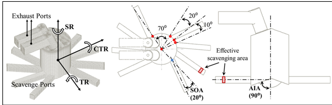
Figure 1. Schematic diagram of the BUSDIG engine design.
