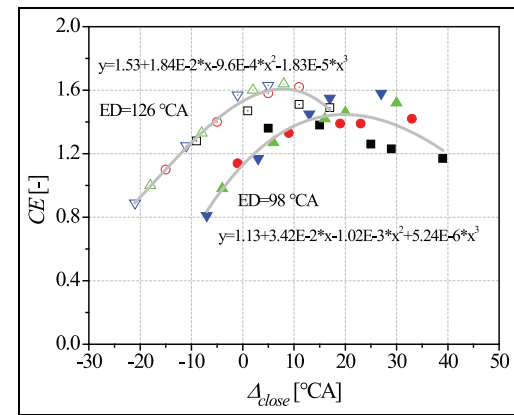
Figure 35. Correlation of CE with \Delta_{close} .
