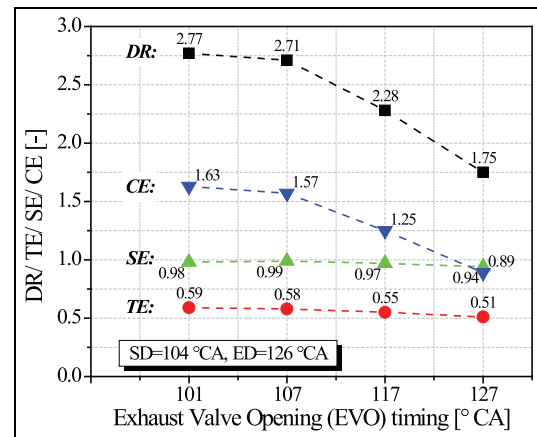
Figure 23. Effect of EVO timing on DR, TE, SE and CE (SD = 104 °CA, ED = 126 °CA).
