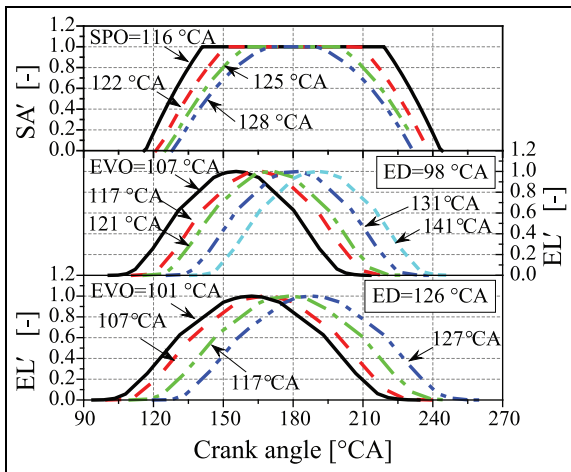
Figure 11. Normalized scavenge port opening area (SA) profiles and exhaust valve lift (EL) profiles.
