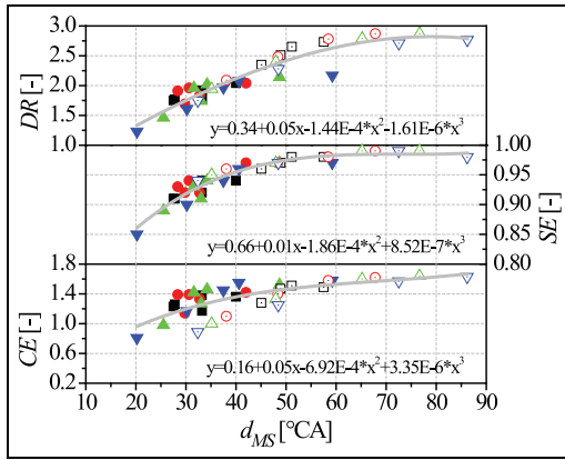
Figure 32. Correlation of DR, SE and CE with d_{MS} .
