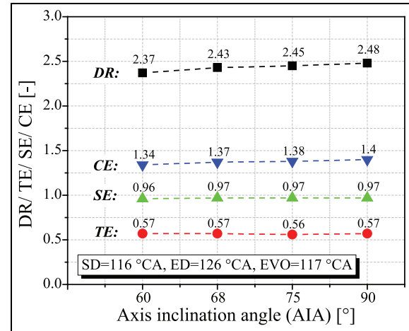
Figure 5. Effect of AIA on DR, TE, SE and CE (SD = 116 °CA, ED = 126 °CA, EVO = 117 °CA).
