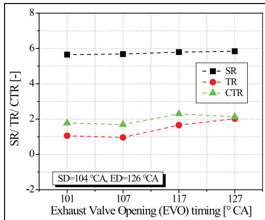
Figure 22. Effect of EVO timing on the SR, TR and CTR at 280 °CA (SD = 104 °CA, ED = 126 °CA).
