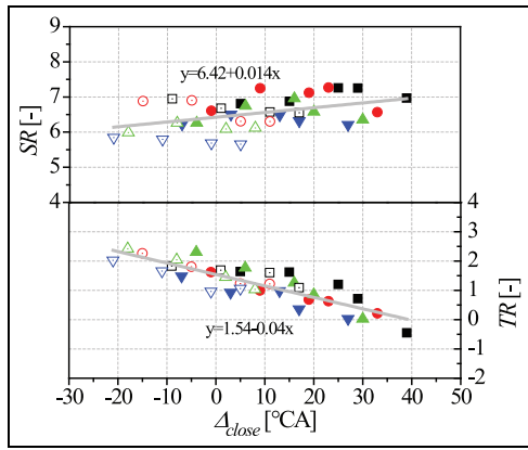
Figure 29. Correlation of SR and TR with \Delta_{close} .
