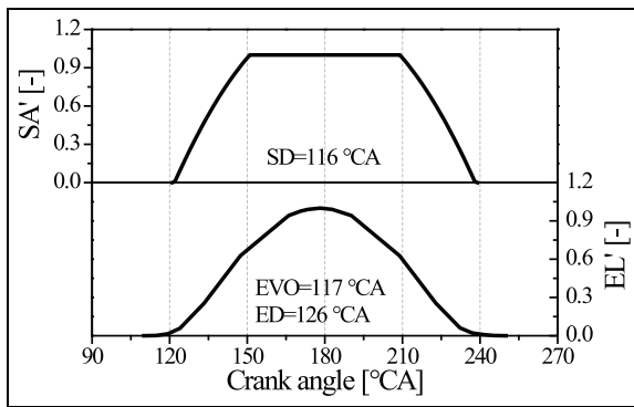
Figure 2. Schematic diagram of the normalized exhaust valve lift profiles (EL') and scavange port opening area (SA') profiles.
