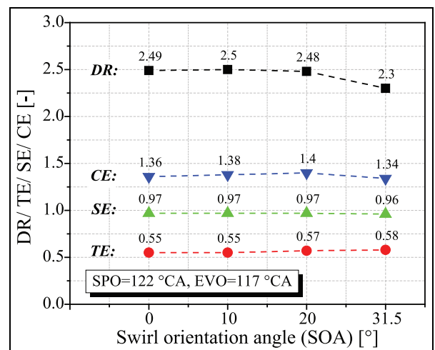
Figure 9. Effect of SOA on DR, TE, SE and CE (SD = 116°CA, ED = 126°CA, EVO = 117°CA).
