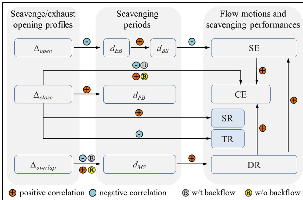
Figure 36. Mechanism of the effect of scavenge port/exhaust valve opening profiles on scavenging periods, in-cylinder flow motions and scavenging performances.
