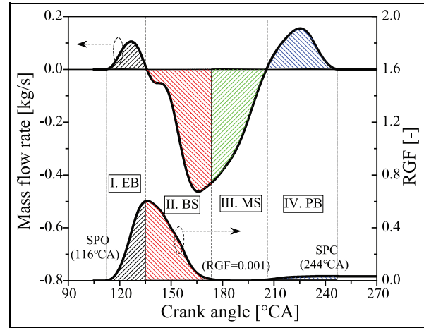
Figure 12. The total mass flow rate and RGF profile at the outlets of scavenge ports, and the definitions of early backflow period (EB), backflow scavenging period (BS), main scavenging period (MS) and post backflow period (PB) (SD = 128 °CA, ED = 98 °CA and EVO = 107 °CA).
