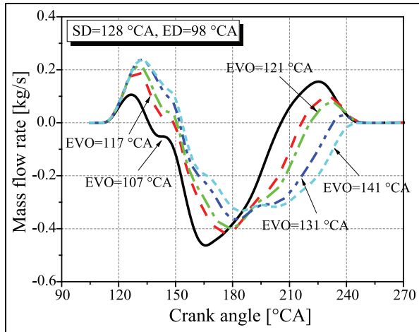
Figure 13. The total mass flow rate profiles at the outlets of scavange ports for different EVOs (SD = 128 °CA, ED = 98 °CA).
