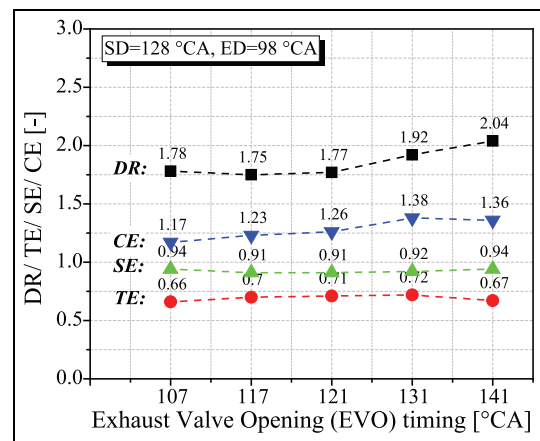
Figure 15. Effect of EVO timing on DR, TE, SE and CE (SD = 128 °CA, ED = 98 °CA).
