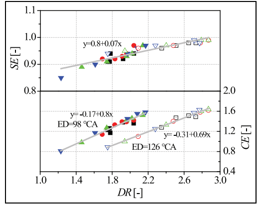
Figure 30. Correlation of SE and CE with DR.
