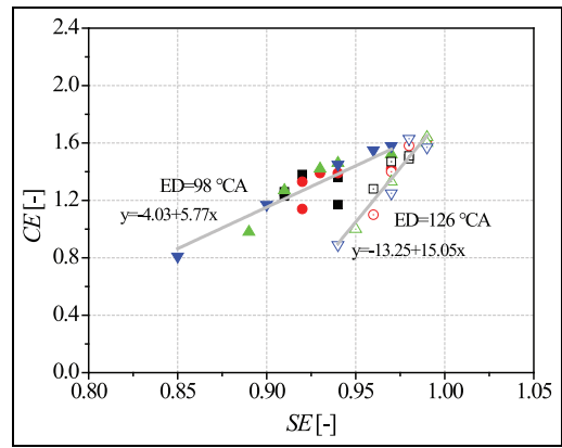
Figure 31. Correlation of CE with SE.
