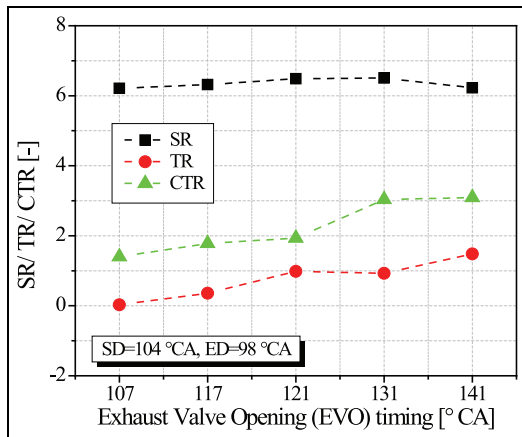
Figure 20. Effect of EVO timing on the SR, TR and CTR at 280 °CA (SD = 104 °CA, ED = 98 °CA).
