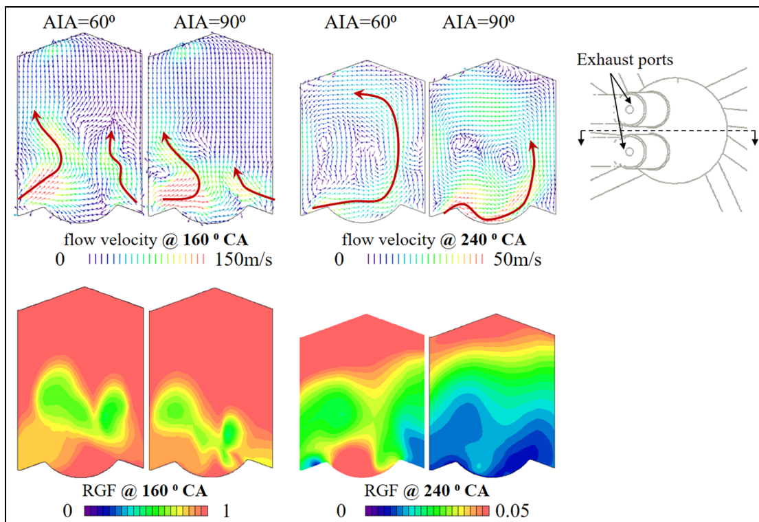
Figure 3. Comparison of the in-cylinder flow field and residual gas fraction (RGF) distribution at 160°CA and 240°CA for AIA = 60° and 90°.
