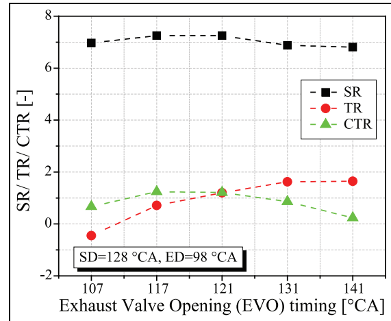
Figure 14. Effect of EVO timing on the SR, TR and CTR at 280 °CA (SD = 128 °CA, ED = 98 °CA).
