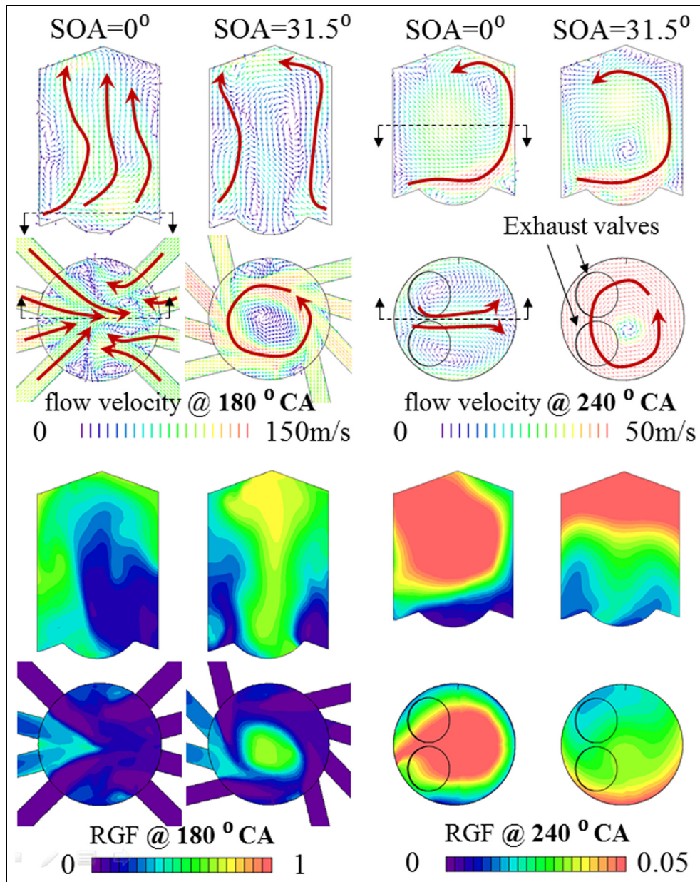
Figure 7. Comparison of the in-cylinder flow field and residual gas fraction (RGF) distribution at 180°CA and 240°CA for SOA = 0° and 31.5°.
