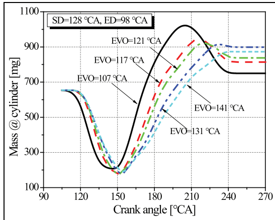
Figure 16. Cylinder mass evolutions with different EVOs (SD = 128 °CA, ED = 98 °CA).
