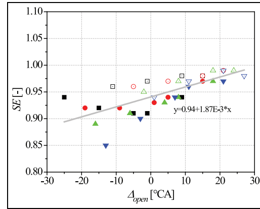
Figure 34. Correlation of SE with \Delta_{open} .
