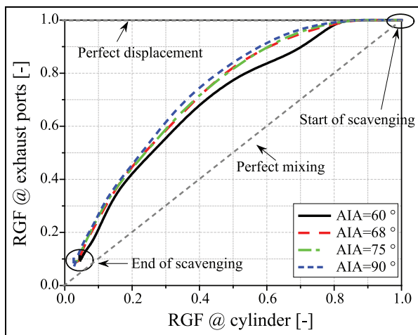
Figure 6. Comparison of RGF profiles in the cylinder and exhaust ports for different AIAs.
