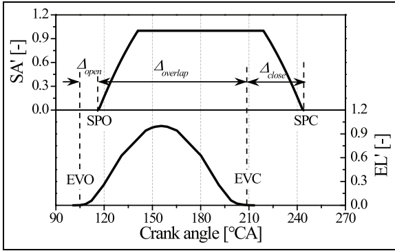
Figure 24. Definitions of \Delta_{open} , \Delta_{close} and \Delta_{overlap} .
