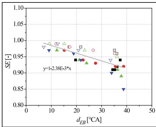
Figure 33. Correlation of SE with d_{EB} .
