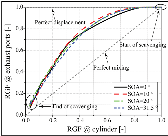
Figure 10. Comparison of RGF profiles in the cylinder and exhaust ports for different SOAs.
