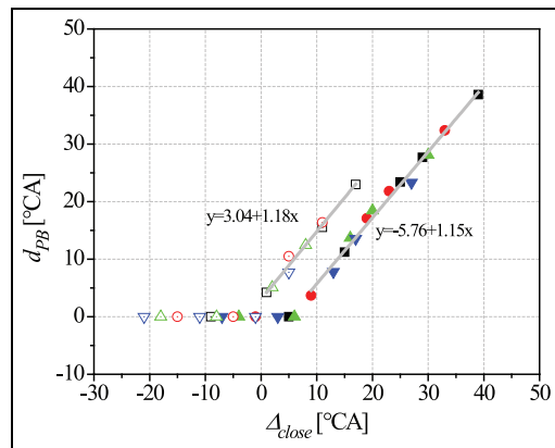
Figure 27. Correlation of d_{PB} with \Delta_{close} .
