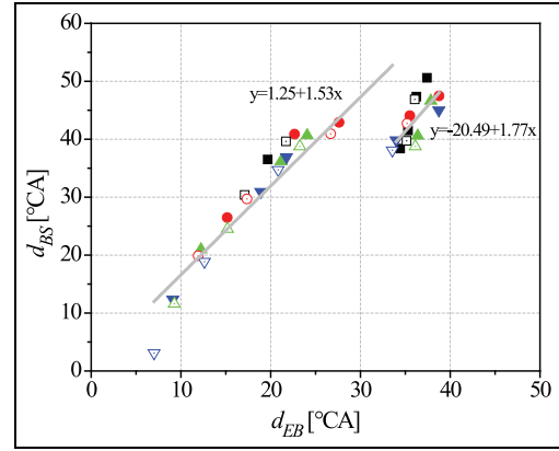
Figure 26. Correlation of d_{BS} with d_{EB} .
