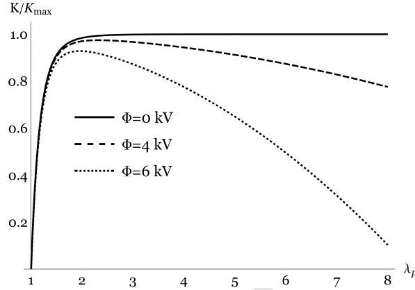
Figure 8. Analytic stiffness response K specialized for the NH model, given by Equ. (22), normalized w.r.t. its value K_{max} \approx 303N/m versus the prestretch \lambda_p , for different values of the applied voltage ( \Phi = 0, 4, 6 kV). The results are obtained for values of the parameters reported in Table 1.
