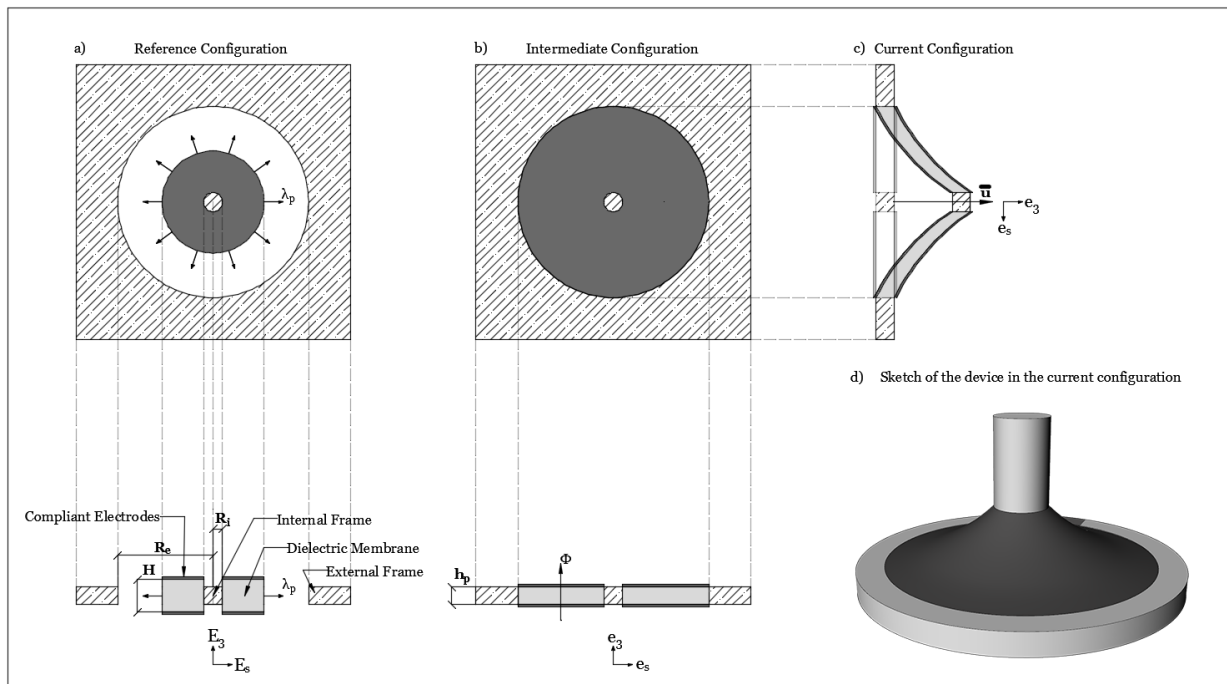
Figure 1. Sketch of the diaphragm device in which an outer rigid frame with inner circular opening of radius R_e is attached to a cylindrical bar of radius R_i through a prestretched ( \lambda_p ) annular DE membrane with initial thickness H and prestretched thickness h_p = H/\lambda_p^2 . In the membrane it is possible to induce a drop voltage \Phi by means of two compliant electrodes. a) Reference configuration, top view above and lateral view in the bottom; b) Intermediate configuration, top view above and lateral view in the bottom; c) Lateral view of the current configuration characterized by a prescribed pulling out displacement \tilde{u} ; d) Sketch of the device in the current configuration.
