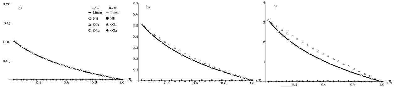
Figure 2. Displacements u_3 and u_s , normalized w.r.t. the width of the annulus w , plotted versus the radial abscissa s normalized w.r.t. the external radius R_e , for values of the prescribed displacement \bar{u} equal to a) 1mm, b) 5mm, c) 30mm. The results are obtained for values of the parameters reported in Table 1, prestretch \lambda_p = 6 and applied drop voltage \Phi = 1kV . For the constitutive model, the following three pairs of elastic coefficients were selected: (NH) \mu_1 = \mu and \mu_2 = 0 , which corresponds to a Neo-Hookean solid; (OG1) \mu_1 = 0 and \mu_2 = \mu/2 ; (OG2) \mu_1 = \mu/2 and \mu_2 = \mu/4 .
