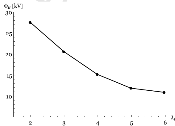
Figure 6. Estimate of the breakdown voltage for the polyacrylate VHB 4910 (3M), for increasing value of prestretch \lambda_p , experimentally obtained by [34] when the elastomer sheet is bi-axially (pre)stretched.
