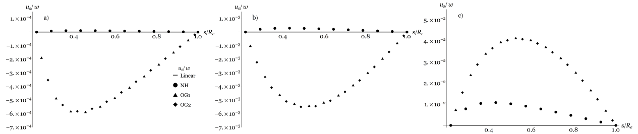
Figure A.9. Displacements u_s , normalized w.r.t. the width of the annulus w , plotted versus the radial abscissa s normalized w.r.t. the external radius R_e , for values of the prescribed displacement \bar{u} equal to a) 1mm, b) 5mm, c) 30mm. The results are obtained for values of the parameters reported in Table 1, prestretch \lambda_p = 6 and applied drop voltage \Phi = 1kV . For the constitutive model, the following three pairs of elastic coefficients were selected: (NH) \mu_1 = \mu and \mu_2 = 0 , which corresponds to a Neo-Hookean solid; (OG1) \mu_1 = 0 and \mu_2 = \mu/2 ; (OG2) \mu_1 = \mu/2 and \mu_2 = \mu/4 .
