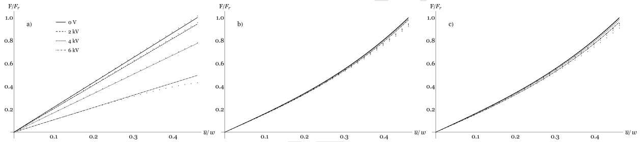
Figure 3. Analytic (solid) and numeric (dotted) response force F normalized w.r.t. its maximum value versus the prescribed displacement \bar{u} normalized w.r.t. the annular width w , for different values of voltage ( \Phi = 0, 2, 4, 6 kV) and for the three constitutive models: a) NH ( \mu_1 = \mu and \mu_2 = 0 ); b) OG1 ( \mu_1 = 0 and \mu_2 = \mu/2 ); c) OG2 ( \mu_1 = \mu/2 and \mu_2 = \mu/4 ). The results are obtained for values of the parameters reported in Table 1 and prestretch \lambda_p = 6 .
