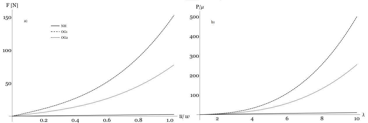
Figure 7. Comparison between (a) the strain response of the device in terms of tensile force F versus the prescribed displacement \bar{u} normalized w.r.t. the annular width w and (b) the strain response in terms of First Piola-Kirchhoff stress P normalized w.r.t. the tangent shear modulus ( \mu ) versus stretch ( \lambda ) in a case of uni-axial stress state. The results are obtained for values of the parameters reported in Table 1, drop voltage \Phi = 3kV and prestretch \lambda_p = 6 . For the constitutive model, the following three pairs of elastic coefficients were selected: (NH) \mu_1 = \mu and \mu_2 = 0 , which corresponds to a Neo-Hookean solid; (OG1) \mu_1 = 0 and \mu_2 = \mu/2 ; (OG2) \mu_1 = \mu/2 and \mu_2 = \mu/4 .
