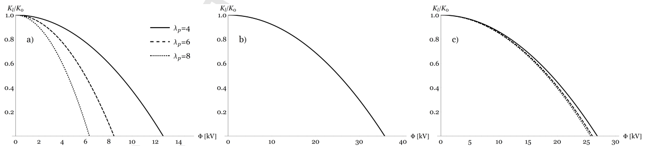
Figure 4. Analytic prediction of the out-of-plane stiffness of the device K_i normalized w.r.t. its value K_0 evaluated for \Phi = 0 versus the applied voltage \Phi for different values of prestretch ( \lambda_p = 4, 6, 8 ), for different values of voltage ( \Phi = 0, 2, 4, 6 kV) and for the three constitutive models: a) NH ( \mu_1 = \mu and \mu_2 = 0 ) which corresponds to K_0 = (302.93 \text{ N/m})(1 - \lambda_p^{-6}) ; b) OG1 ( \mu_1 = 0 and \mu_2 = \mu/2 ) which corresponds to K_0 = (151.46 \text{ N/m})(\lambda_p^2 - \lambda_p^{-10}) ; c) OG2 ( \mu_1 = \mu/2 and \mu_2 = \mu/4 ) which corresponds to K_0 = (151.46 \text{ N/m})(1 - \lambda_p^{-6}) + (75.73 \text{ N/m})(\lambda_p^2 - \lambda_p^{-10}) . The results are obtained for values of the parameters reported in Table 1.
