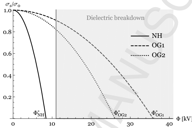
Figure 5. Radial stress \sigma_s normalized w.r.t. the membrane stress \sigma_0 at \Phi = 0 versus the applied voltage for the three constitutive models: a) NH ( \mu_1 = \mu and \mu_2 = 0 ) which corresponds to \sigma_0 = 2.63 \text{ MPa} ; b) OG1 ( \mu_1 = 0 and \mu_2 = \mu/2 ) which corresponds to \sigma_0 = 47.30 \text{ MPa} ; c) OG2 ( \mu_1 = \mu/2 and \mu_2 = \mu/4 ) which corresponds to 24.97 \text{ MPa} , highlighting the region in which the dielectric breakdown occurs (gray region). The critical voltage \Phi^* , at which the stress vanishes, is \approx 8, 35, 26 \text{ kV} for the NH, OG1, and OG2 model, respectively. The results are obtained for values of the parameters reported in Table 1 and prestretch \lambda_p = 6 .
