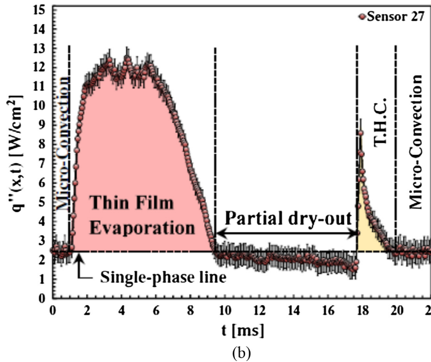
Fig. 10. Motion and growth of the elongated bubble due to evaporation (a) and the instantaneous heat flux and heat transfer mechanisms during the passage of the elongated bubble over the temperature sensor (b), Bigham and Moghaddam [72]; T.H.C. (transient heat conduction).
