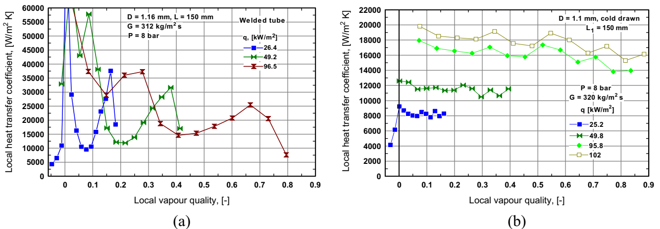
Fig. 14. The local heat transfer coefficient versus local vapour quality for (a) the welded tube and (b) the cold drawn tube, adapted from Karayiannis et al. [93].
