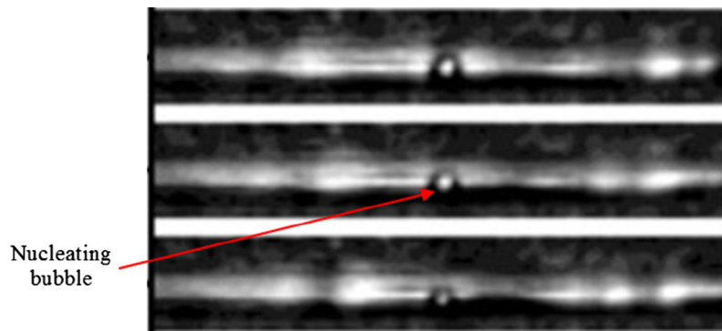
Fig. 9. Nucleation in the annular liquid film, Borhani and Thome [69].
