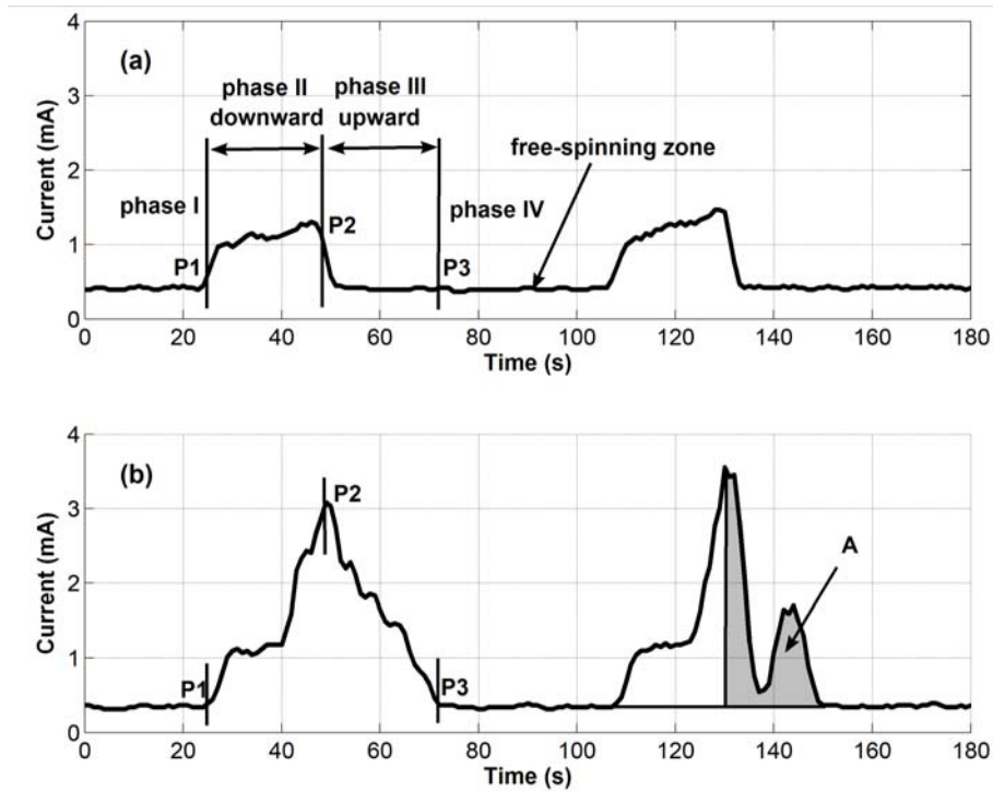
Figure 1. A sample of recorded signal; (a) coated drill after drilling 270 holes, (b) uncoated drill close to failure. P1-P3 represents key points in the signal and A is the area under current curve in phase III.
