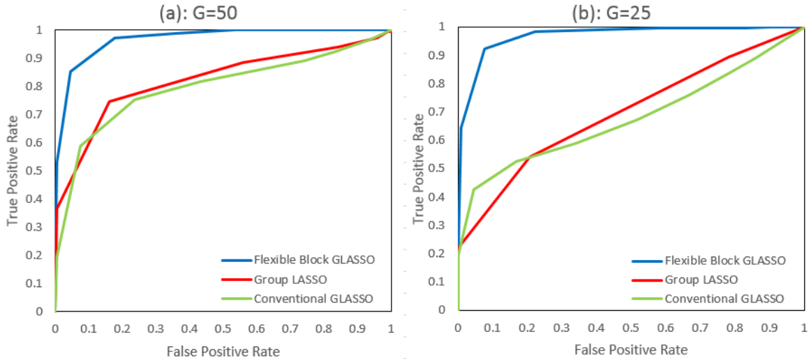
Figure 2: Flexible Block-GLASSO vs Group LASSO and conventional GLASSO in the case of within-block variation, for N = 100 , T = 200 and G = 50 (left) and G = 25 (right).
