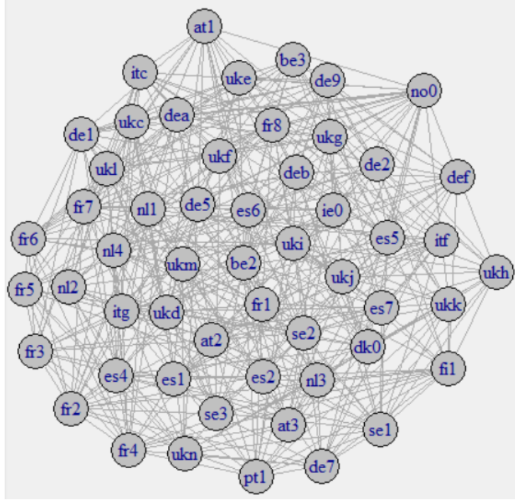
Figure 3: Adjacency graph of per-capita GVA growth, 1980-2012 estimated via Block-GLASSO, taking the NUTS1 regions as blocks.
