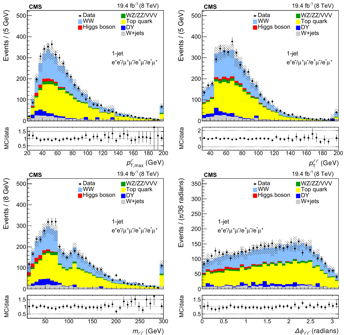
Fig. 2 The data and MC distributions for the one-jet category of the leading lepton p_T ( p_{T, \max}^{\ell} ), the p_T of the dilepton system ( p_T^{\ell\ell} ), the dilepton invariant mass ( m_{\ell\ell} ) and the azimuthal angle between the two leptons ( \Delta\phi_{\ell\ell} ). The hatched areas represent the total systematic uncer-
