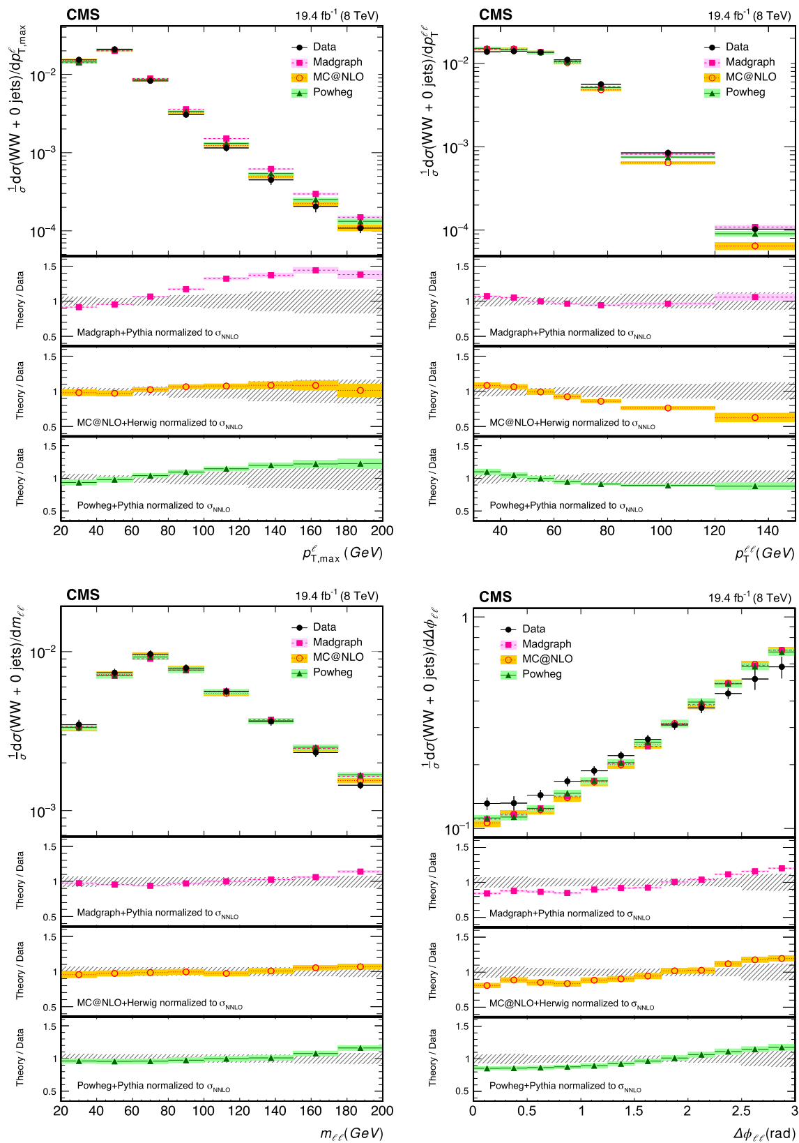
Fig. 3 Normalized differential W^+W^- cross section as a function of the leading lepton p_T ( p_{T, \max}^\ell ) (top left), the transverse momentum of the dilepton system ( p_T^{\ell\ell} ) (top right), the invariant mass ( m_{\ell\ell} ) (bottom left) and the angular separation between leptons ( \Delta\phi_{\ell\ell} ) (bottom right).
