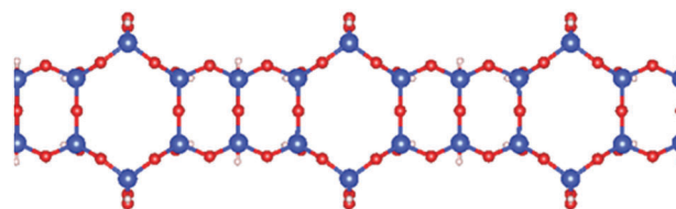
Fig. 7 Schematic picture of the optimized structure of one 1D SNR decorated with both hexagonal rings and squares.
