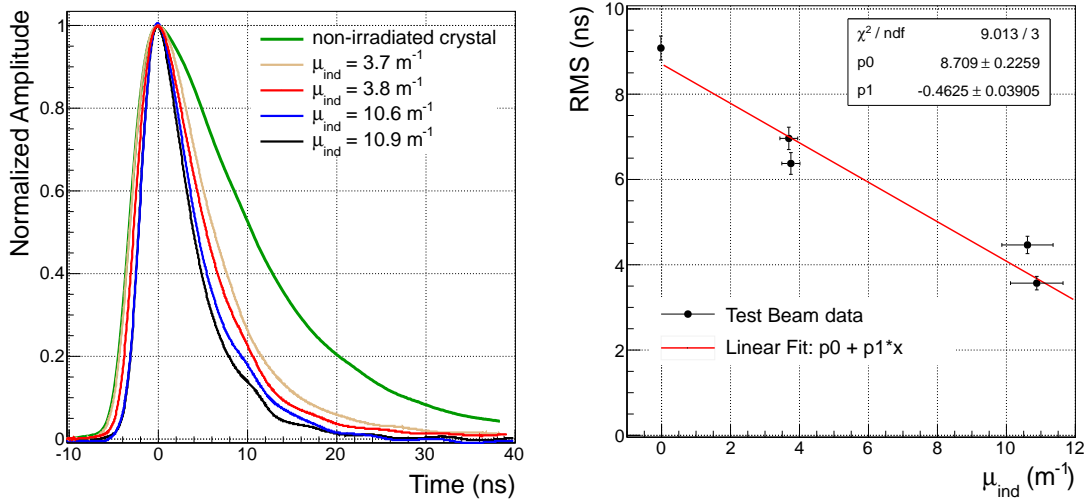
Figure 19. Left: waveforms of a non-irradiated crystal and four proton-irradiated crystals are shown. The \mu_{\text{ind}} of the irradiated crystals varies between 3.7 \text{ m}^{-1} and 10.9 \text{ m}^{-1} . Right: correlation between \mu_{\text{ind}} and RMS of the average pulse fitted with a linear function (red).
