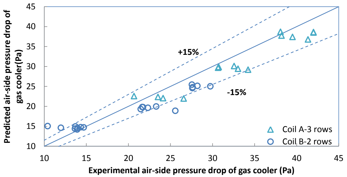
Fig. 8. Comparison of simulation and experimental results for air side pressure drops of gas coolers
