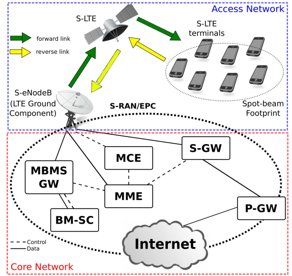
Fig. 1. The Satellite-LTE reference scenario
