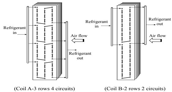
Fig. 4 two tested finned-tube CO 2 gas coolers/condensers
