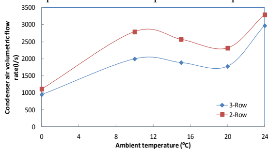
Fig. 5 variation of volumetric flow rate with ambient temperature for different CO 2 condensers
