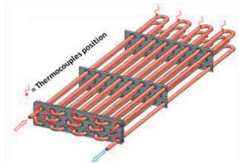
Fig. 2 pipe arrangement and thermocouple locations
