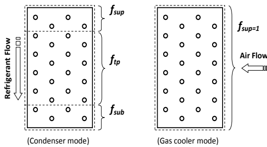
Fig. 3 single circuit heat exchanger and segment divisions
