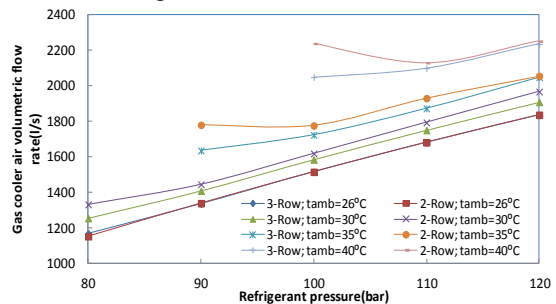
Fig. 6 variation of volumetric flow rate with ambient temperature and supercritical pressure for different CO 2 gas cooler
