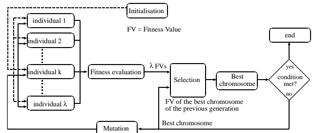
Figure 1. Implemented algorithm for the design and optimization of digital logic circuits. Figure taken from [7].
