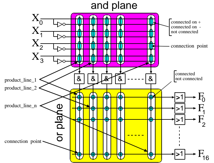
Figure 2. Schema of the PLA with representation of the chromosome.
