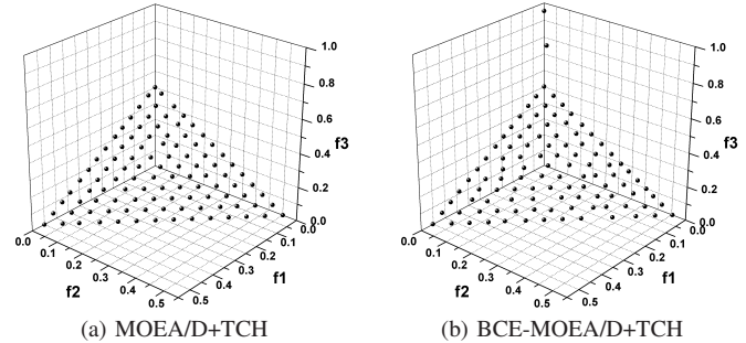
Fig. 19. The final solution set of MOEA/D+TCH and BCE-MOEA/D+TCH on DTLZ1.
