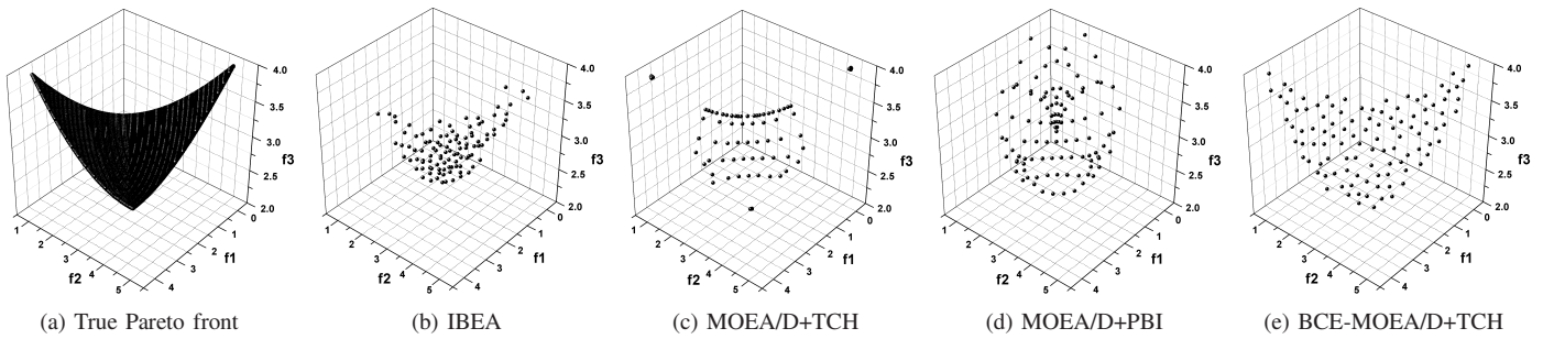
Fig. 5. True Pareto front and the final solution set on VNT1, where the solutions of the three BCE algorithms have similar distribution.
