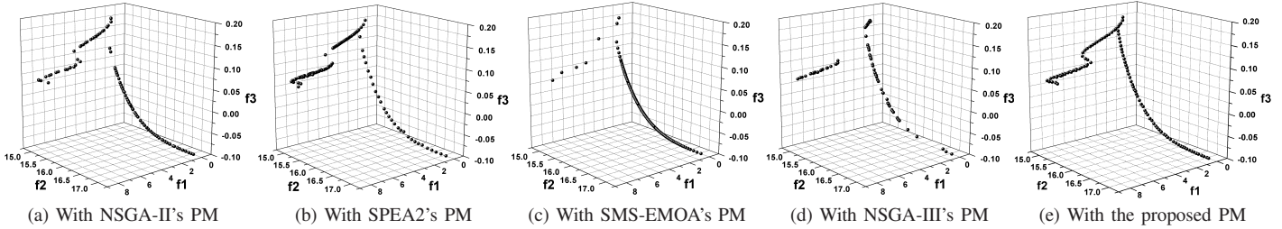
Fig. 17. The solution sets obtained by BCE-MOEA/D+TCH with different population maintenance (PM) methods on VNT3.
