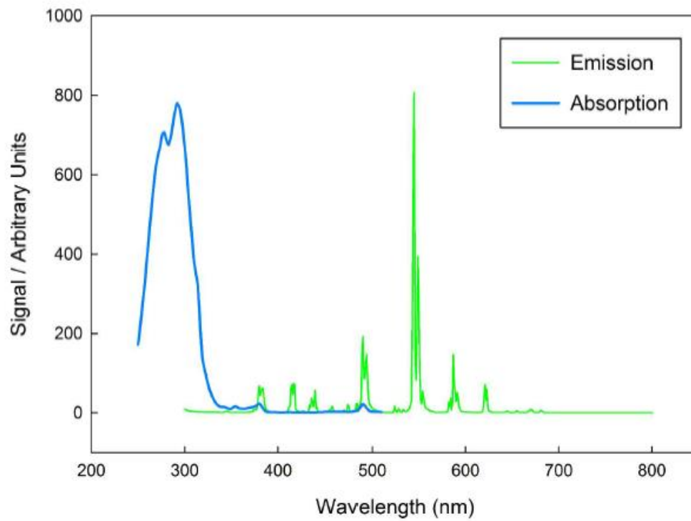
Figure 4. PLE and PL of \text{Gd}_2\text{O}_2\text{S}(\text{Er}_{0.2},\text{Tb})_{0.01} at room temperature. 902x664mm (96 x 96 DPI)
