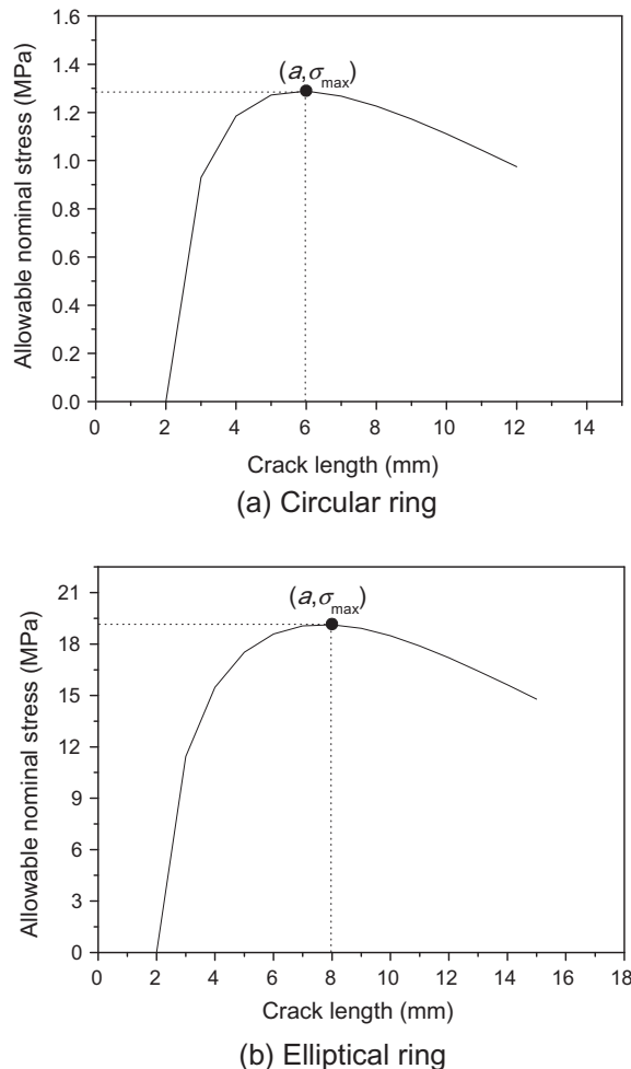
Fig. 11. Allowable nominal stress in concrete rings from fracture analysis.
