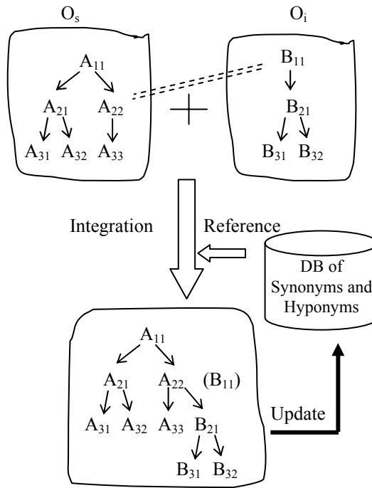
Figure 5. Ontology integration
