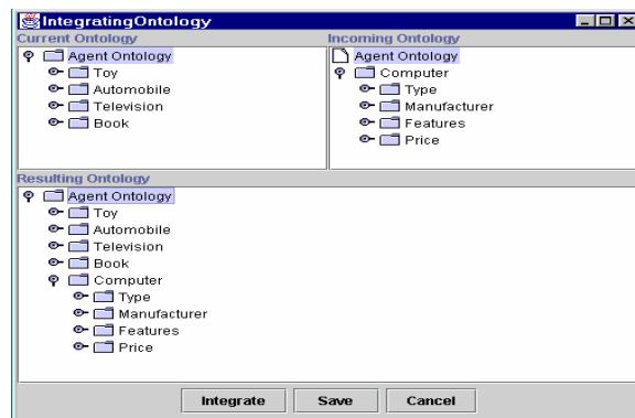
Figure 7. A screenshot of integrating ontology
