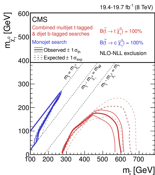
Figure 9. Expected and observed 95% CL exclusion limits in the (m_{\tilde{\tau}}, m_{\tilde{\chi}_1^0}) mass plane for top-squark pair production, assuming 100% branching fraction to the decay \tilde{\tau} \rightarrow t\tilde{\chi}_1^0 , or, in the case of a highly compressed spectrum, to \tilde{\tau} \rightarrow c\tilde{\chi}_1^0 . The \pm 1\sigma_{\text{exp}} and \pm 1\sigma_{\text{th}} limit curves are also shown. The combined results from the dijet b-tagged and multijet t-tagged searches and the result from the monojet search are displayed separately. The dashed black diagonal lines mark the borders of the various kinematic regimes leading to different top squark decays as described in the text.
