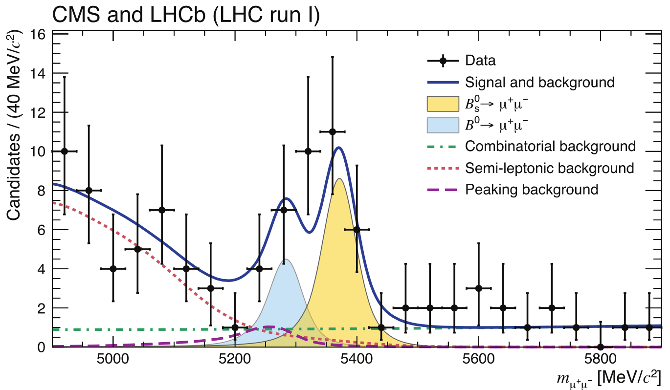
Extended Data Figure 2 | Distribution of the dimuon invariant mass m_{\mu^+\mu^-} for the best six categories. Categories are ranked according to values of S/(S + B) where S and B are the numbers of signal events expected assuming the SM rates and background events under the B_s^0 peak for a given category, respectively. The mass distribution for the six highest-ranking categories, three
