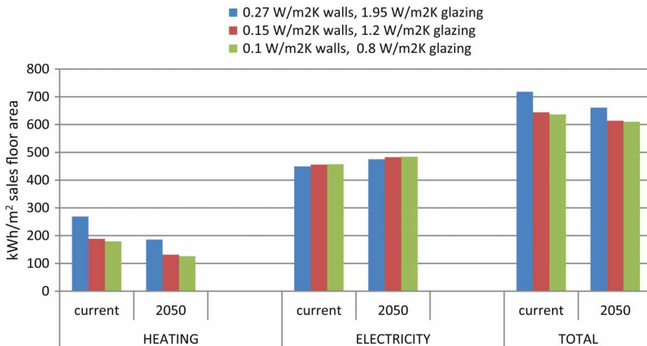
Figure 9. Effect of reduction of envelope (first number) and glazing (second number) heat transfer ( \text{W}/\text{m}^2\text{K} , U -values) on heating and electricity energy demand for current and 2050s weather data.
