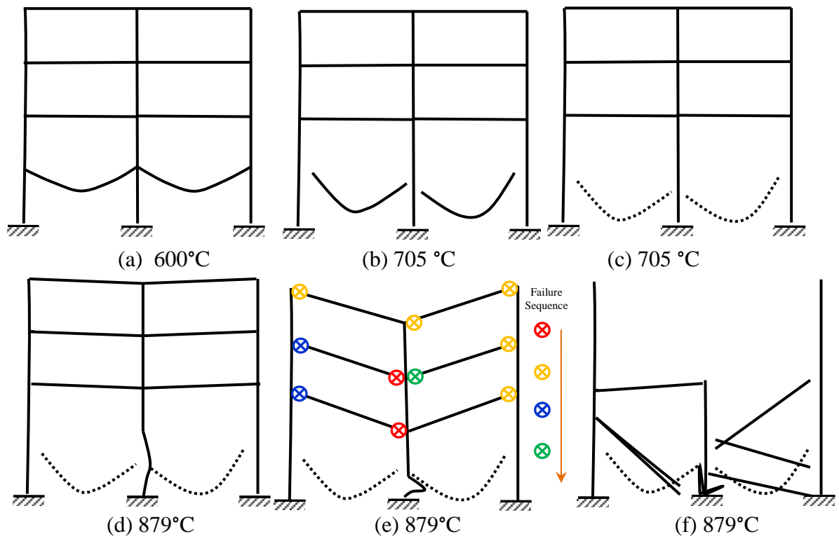
Fig. 18. Collapse sequence of Frame 1.
