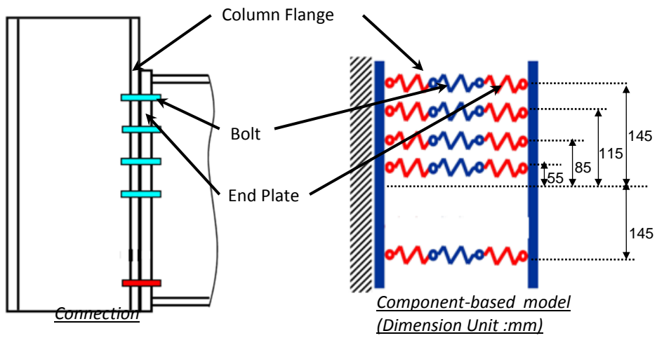
Fig. 20. Endplate connection at J1 and J2 (see Fig. 3), and its component-based model.
