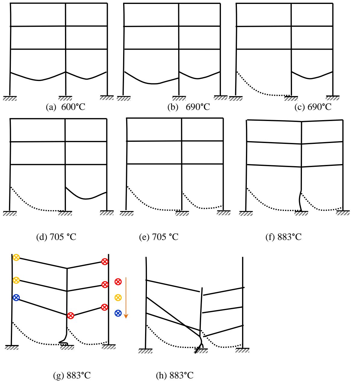
Fig. 21. Collapse sequence of Frame 2.
