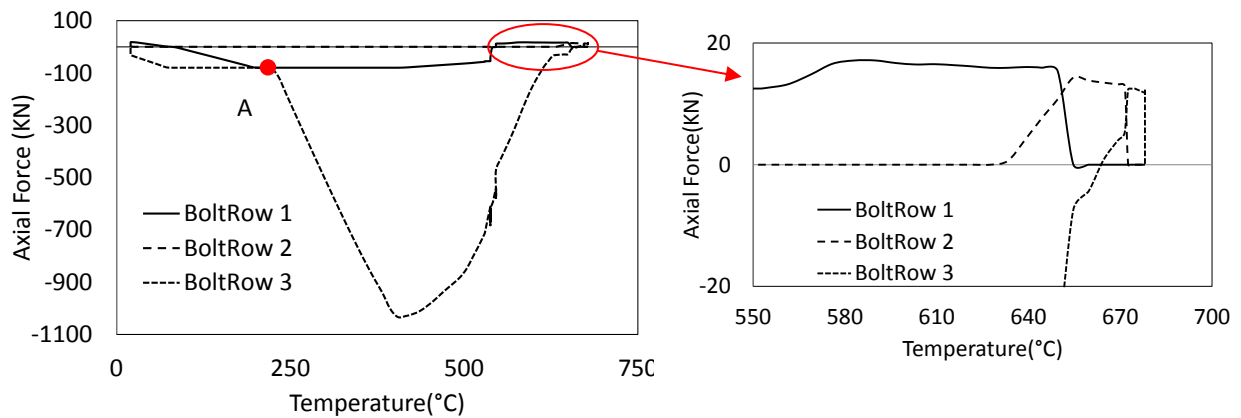
Fig. 12. Axial forces in the components in connection of Type 1 (Frame 1)
