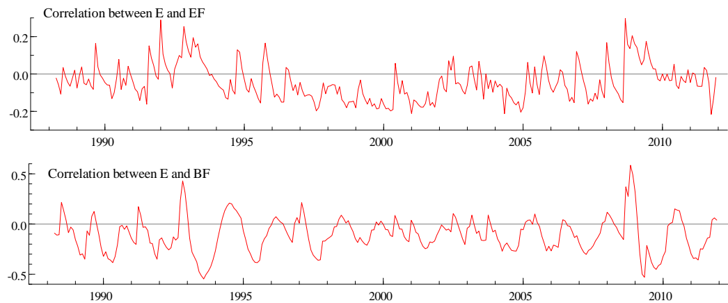
Fig. 2 (continued). The evolution of the dynamic conditional correlations between exchange rate changes ( E_t ) and net equity ( EF_t ) and net bond flows ( BF_t ) (calculated as h_{12} / \sqrt{h_{11,t}} \sqrt{h_{22,t}} ).
